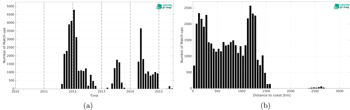
Figure 2: Number of match-ups between Surface drifters and Aquarius SSS L4 OI v5 - Weekly (IPRC) SSS as a function of time (a) and as function of the distance to coast (b) over the Equatorial Ocean 10N-10S Pi-MEP region and for the full satellite product period.
