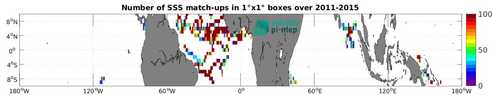
Figure 4: Number of SSS match-ups between Surface drifters SSS and the Aquarius SSS L4 OI v5 - Weekly (IPRC) SSS product for the Equatorial Ocean 10N-10S Pi-MEP region over 1^\circ \times 1^\circ boxes and for the full satellite product period.
