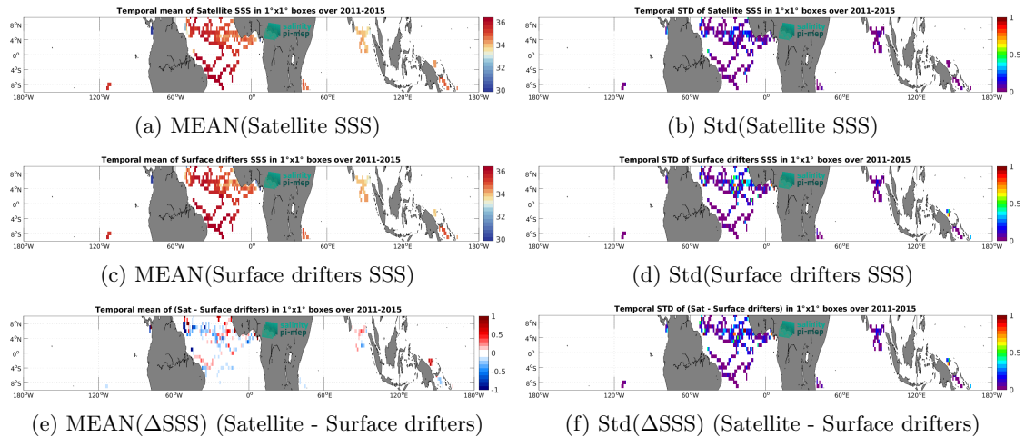
Figure 6: Temporal mean (left) and Std (right) of SSS from Aquarius SSS L4 OI v5 - Weekly (IPRC) (top), Surface drifters (middle), and of \Delta SSS (Satellite - Surface drifters). Only match-up pairs are used to generate these maps.
