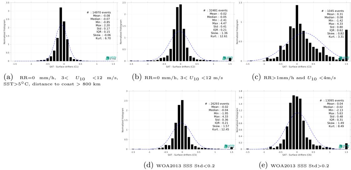
Figure 14: Normalized histogram of \Delta SSS (Aquarius SSS L4 OI v5 - Weekly (IPRC) - Surface drifters) for 5 different subdatasets corresponding to: RR=0 mm/h, 3 < U_{10} < 12 m/s, SST >5^\circ C, distance to coast > 800 km (a), RR=0 mm/h, 3 < U_{10} < 12 m/s (b), RR >1 mm/h and U_{10} < 4 m/s (c), WOA2013 SSS Std <0.2 (d), WOA2013 SSS Std >0.2 (e).
