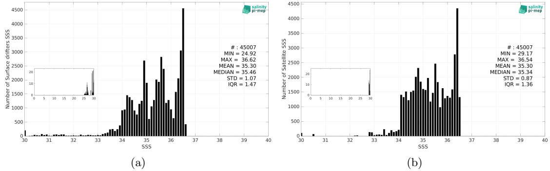
Figure 3: Histograms of SSS from Surface drifters (a) and Aquarius SSS L4 OI v5 - Weekly (IPRC) (b) considering all match-up pairs per bins of 0.1 over the Equatorial Ocean 10N-10S Pi-MEP region and for the full satellite product period.
