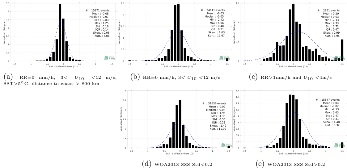
Figure 12: Normalized histogram of \Delta SSS (Aquarius SSS L4 OI v5 - Weekly (IPRC) - Surface drifters) for 5 different subdatasets corresponding to: RR=0 mm/h, 3 < U_{10} < 12 m/s, SST > 5^\circ C , distance to coast > 800 km (a), RR=0 mm/h, 3 < U_{10} < 12 m/s (b), RR >1 mm/h and U_{10} < 4 m/s (c), WOA2013 SSS Std <0.2 (d), WOA2013 SSS Std >0.2 (e).
