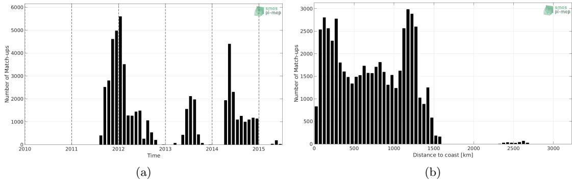
Figure 1: Number of match-ups between Surface drifters and Aquarius-L4-IPRC-V5-WEEKLY SSS as a function of time (a) and as function of the distance to coast (b) over the Equatorial Ocean 10N-10S Pi-MEP region and for the full satellite product period.
