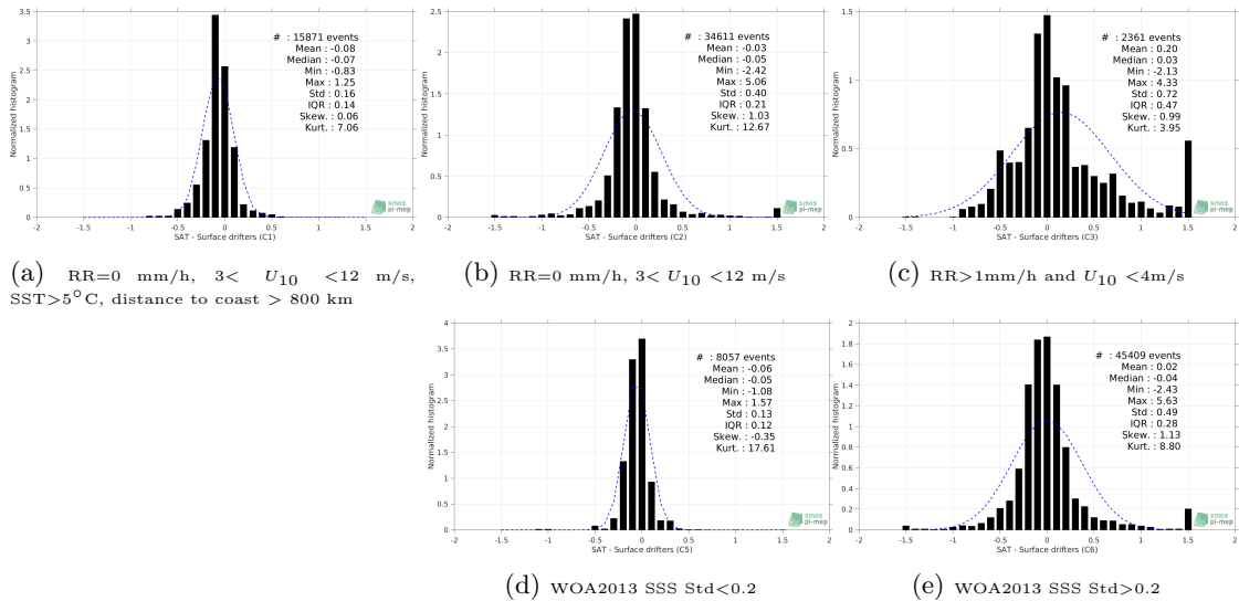
Figure 12: Normalized histogram of ΔSSS (Aquarius-L4-IPRC-V5-WEEKLY - Surface drifters) for 5 different subdatasets corresponding to: RR=0 mm/h, 3 < U_{10} < 12 m/s, SST > 5°C, distance to coast > 800 km (a), RR=0 mm/h, 3 < U_{10} < 12 m/s (b), RR > 1mm/h and U_{10} < 4m/s (c), WOA2013 SSS Std < 0.2 (d), WOA2013 SSS Std > 0.2 (e).
