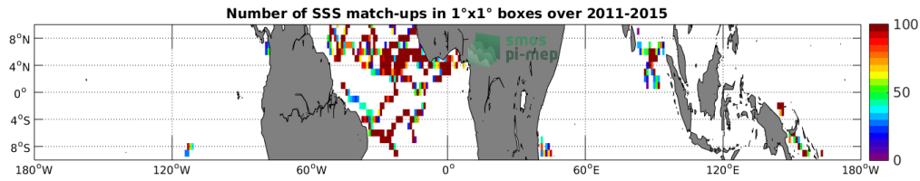
Figure 3: Number of SSS match-ups between Surface drifters SSS and the Aquarius-L4-IPRC-V5-WEEKLY SSS product for the Equatorial Ocean 10N-10S Pi-MEP region over 1^\circ \times 1^\circ boxes and for the full satellite product period.
