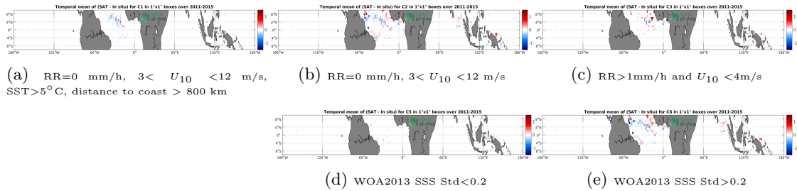
Figure 11: Temporal mean gridded over spatial boxes of size 1°x1° of \Delta SSS (Aquarius-L4-IPRC-V5-WEEKLY - Surface drifters) for 5 different subdatasets corresponding to:RR=0 mm/h, 3 < U_{10} < 12 m/s, SST>5°C, distance to coast > 800 km (a), RR=0 mm/h, 3 < U_{10} < 12 m/s (b), RR>1mm/h and U_{10} < 4m/s (c), WOA2013 SSS Std<0.2 (d), WOA2013 SSS Std>0.2 (e).
