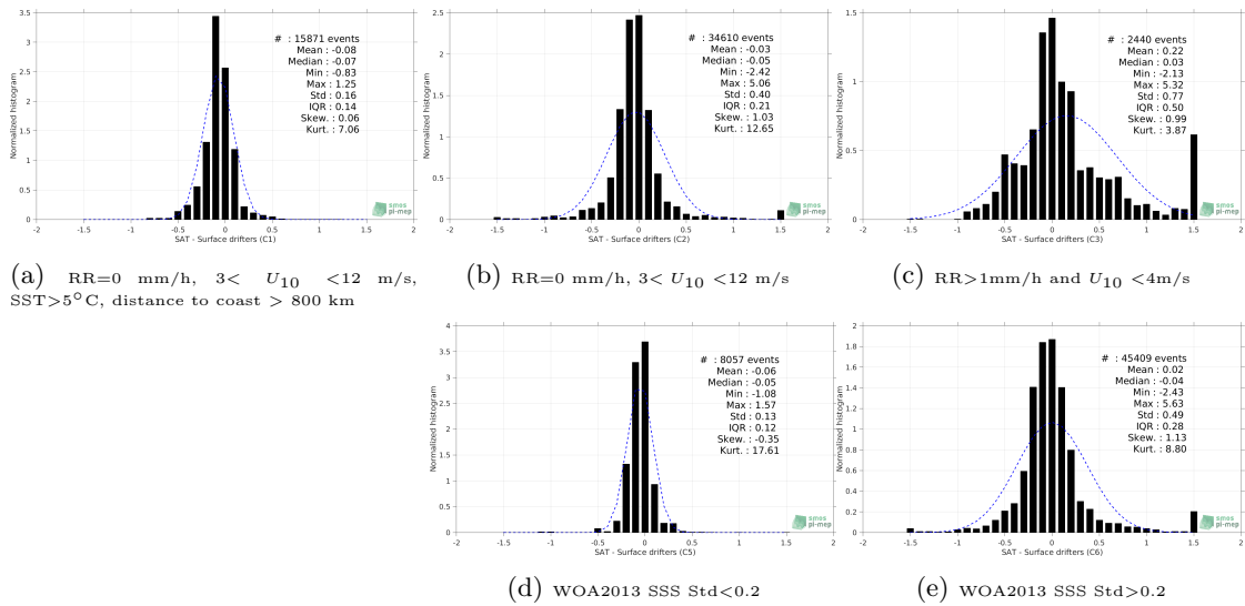
Figure 12: Normalized histogram of \Delta SSS (Aquarius-L4-IPRC-V5-WEEKLY - Surface drifters) for 5 different subdatasets corresponding to: RR=0 mm/h, 3 < U_{10} < 12 m/s, SST >5^\circ\text{C} , distance to coast > 800 km (a), RR=0 mm/h, 3 < U_{10} < 12 m/s (b), RR >1 mm/h and U_{10} < 4 m/s (c), WOA2013 SSS Std <0.2 (d), WOA2013 SSS Std >0.2 (e).
