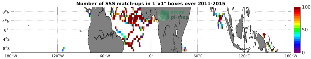
Figure 3: Number of SSS match-ups between Surface drifters SSS and the Aquarius-L4-IPRC-V5-WEEKLY SSS product for the Equatorial Ocean 10N-10S Pi-MEP region over 1^\circ \times 1^\circ boxes and for the full satellite product period.
