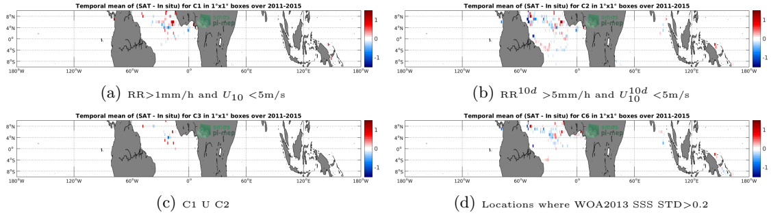
Figure 11: Temporal mean gridded over spatial boxes of size 1^\circ \times 1^\circ of \Delta SSS (Aquarius-L4-IPRC-V5-WEEKLY - Surface drifters) for 4 different subdatasets corresponding to: RR >1 mm/h and U_{10} < 5 m/s (a), RR ^{10d} > 5 mm/h and U_{10}^{10d} < 5 m/s (b), C1 U C2 (c), Locations where WOA2013 SSS STD >0.2 (d).
