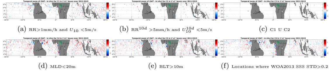
Figure 12: Temporal mean gridded over spatial boxes of size 1^\circ \times 1^\circ of \Delta\text{SSS} (Aquarius-L4-IPRC-V5-WEEKLY - Argo) for 6 different subdatasets corresponding to: \text{RR} > 1\text{mm/h} and U_{10} < 5\text{m/s} (a), \text{RR}^{10d} > 5\text{mm/h} and U_{10}^{10d} < 5\text{m/s} (b), C1 U C2 (c), \text{MLD} < 20\text{m} (d), \text{BLT} > 10\text{m} (e), Locations where WOA2013 SSS \text{STD} > 0.2 (f).
