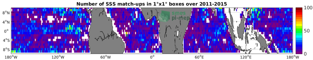
Figure 4: Number of SSS match-ups between Argo SSS and the Aquarius-L4-IPRC-V5-WEEKLY SSS product for the Equatorial Ocean 10N-10S Pi-MEP region over 1°x1° boxes and for the full satellite product period.
