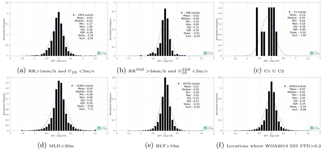
Figure 13: Normalized histogram of \Delta\text{SSS} (Aquarius-L4-IPRC-V5-WEEKLY - Argo) for 6 different subdatasets corresponding to: \text{RR} > 1\text{mm/h} and U_{10} < 5\text{m/s} (a), \text{RR}^{10d} > 5\text{mm/h} and U_{10}^{10d} < 5\text{m/s} (b), C1 U C2 (c), \text{MLD} < 20\text{m} (d), \text{BLT} > 10\text{m} (e), Locations where WOA2013 SSS \text{STD} > 0.2 (f).
