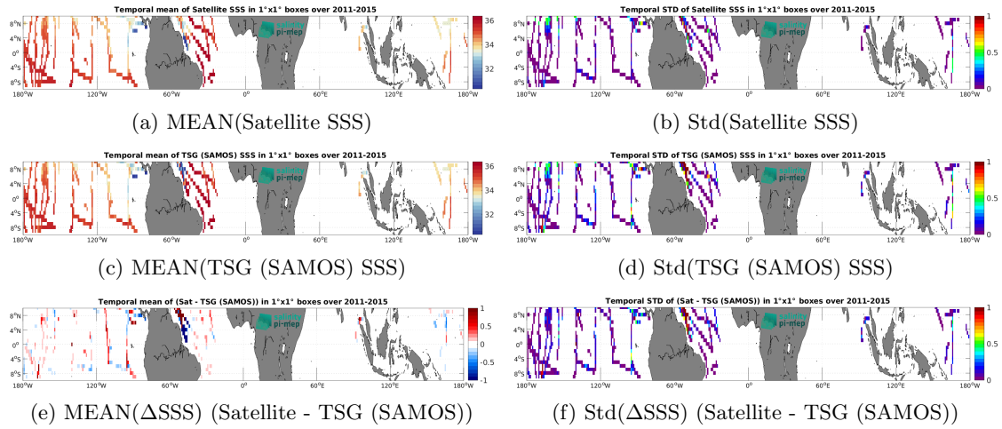
Figure 7: Temporal mean (left) and Std (right) of SSS from Aquarius SSS L4 OI v5 - Monthly (IPRC) (top), TSG (SAMOS) (middle), and of \Delta SSS (Satellite - TSG (SAMOS)). Only match-up pairs are used to generate these maps.
