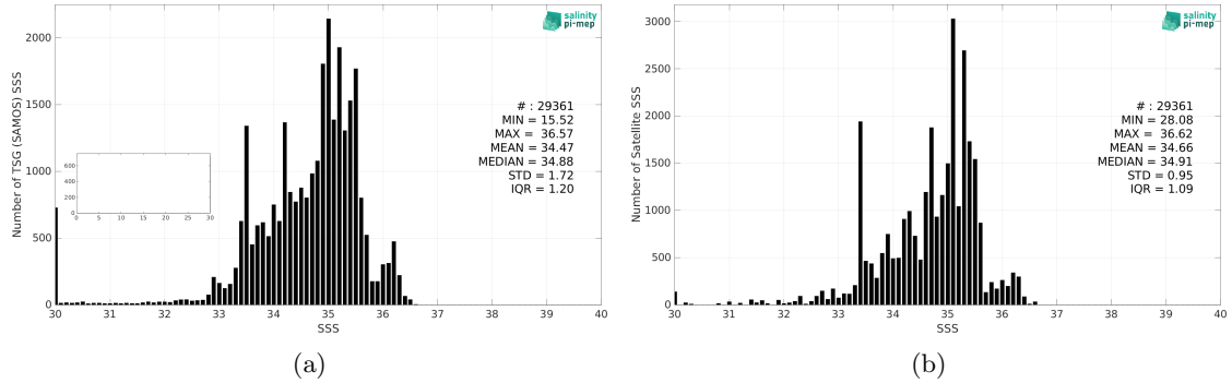
Figure 2: Histograms of SSS from TSG (SAMOS) (a) and Aquarius SSS L4 OI v5 - Monthly (IPRC) (b) considering all match-up pairs per bins of 0.1 over the Equatorial Ocean 10N-10S Pi-MEP region and for the full satellite product period.
