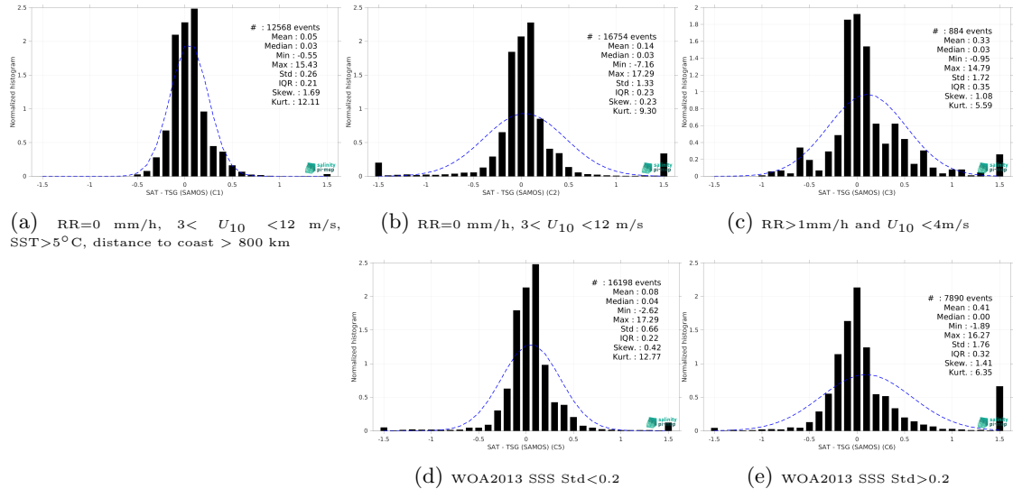
Figure 13: Normalized histogram of \Delta SSS (Aquarius SSS L4 OI v5 - Monthly (IPRC) - TSG (SAMOS)) for 5 different subdatasets corresponding to: RR=0 mm/h, 3 < U_{10} < 12 m/s, SST >5^\circ C, distance to coast > 800 km (a), RR=0 mm/h, 3 < U_{10} < 12 m/s (b), RR >1 mm/h and U_{10} < 4 m/s (c), WOA2013 SSS Std <0.2 (d), WOA2013 SSS Std >0.2 (e).
