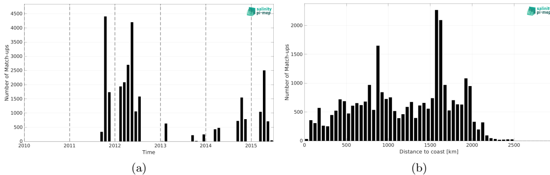
Figure 1: Number of match-ups between TSG (SAMOS) and Aquarius SSS L4 OI v5 - Monthly (IPRC) SSS as a function of time (a) and as function of the distance to coast (b) over the Equatorial Ocean 10N-10S Pi-MEP region and for the full satellite product period.
