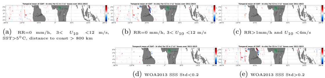
Figure 12: Temporal mean gridded over spatial boxes of size 1°x1° of \Delta SSS (Aquarius SSS L4 OI v5 - Monthly (IPRC) - TSG (SAMOS)) for 5 different subdatasets corresponding to:RR=0 mm/h, 3 < U_{10} < 12 m/s, SST>5°C, distance to coast > 800 km (a), RR=0 mm/h, 3 < U_{10} < 12 m/s (b), RR>1mm/h and U_{10} < 4 m/s (c), WOA2013 SSS Std<0.2 (d), WOA2013 SSS Std>0.2 (e).
