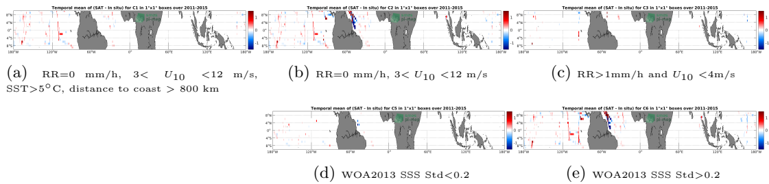
Figure 12: Temporal mean gridded over spatial boxes of size 1°x1° of \Delta SSS (Aquarius SSS L4 OI v5 - Monthly (IPRC) - TSG (SAMOS)) for 5 different subdatasets corresponding to:RR=0 mm/h, 3 < U_{10} < 12 m/s, SST>5°C, distance to coast > 800 km (a), RR=0 mm/h, 3 < U_{10} < 12 m/s (b), RR>1mm/h and U_{10} < 4m/s (c), WOA2013 SSS Std<0.2 (d), WOA2013 SSS Std>0.2 (e).
