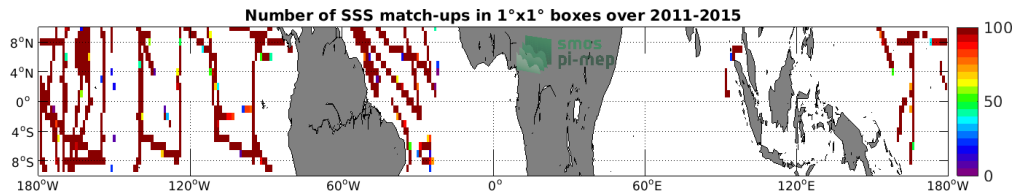
Figure 4: Number of SSS match-ups between TSG (SAMOS) SSS and the Aquarius SSS L4 OI v5 - Monthly (IPRC) SSS product for the Equatorial Ocean 10N-10S Pi-MEP region over 1°x1° boxes and for the full satellite product period.
