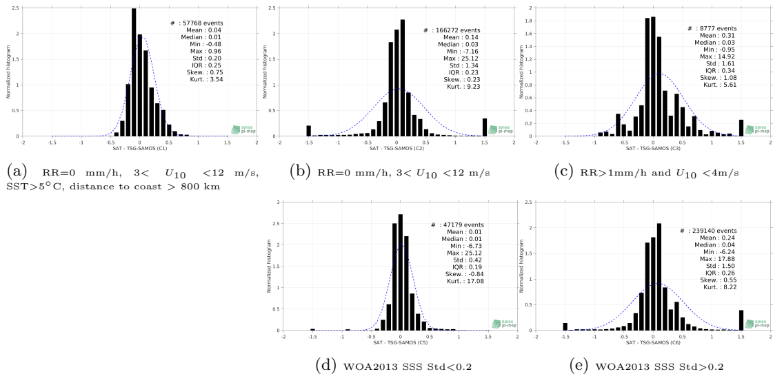
Figure 13: Normalized histogram of \Delta SSS (Aquarius-L4-IPRC-V5-MONTHLY - TSG-SAMOS) for 5 different subdatasets corresponding to: RR=0 mm/h, 3 < U_{10} < 12 m/s, SST >5^\circ\text{C} , distance to coast > 800 km (a), RR=0 mm/h, 3 < U_{10} < 12 m/s (b), RR >1 mm/h and U_{10} < 4 m/s (c), WOA2013 SSS Std <0.2 (d), WOA2013 SSS Std >0.2 (e).
