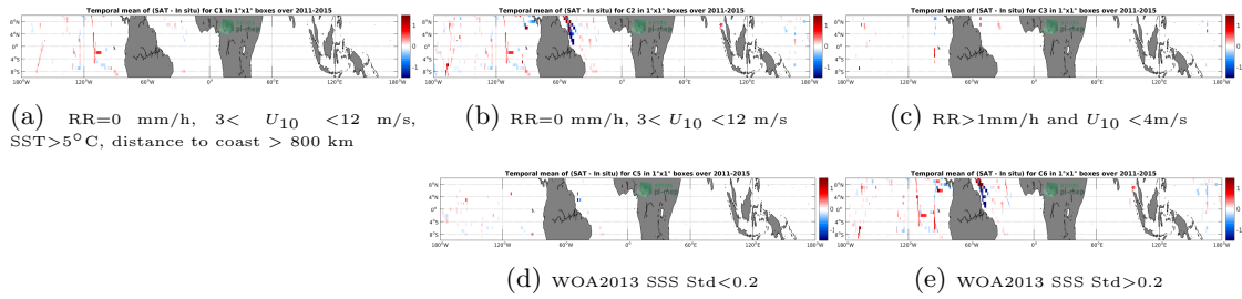
Figure 12: Temporal mean gridded over spatial boxes of size 1^\circ \times 1^\circ of \Delta SSS (Aquarius-L4-IPRC-V5-MONTHLY - TSG-SAMOS) for 5 different subdatasets corresponding to: RR=0 mm/h, 3 < U_{10} < 12 m/s, SST >5^\circ\text{C} , distance to coast > 800 km (a), RR=0 mm/h, 3 < U_{10} < 12 m/s (b), RR >1 mm/h and U_{10} < 4 m/s (c), WOA2013 SSS Std <0.2 (d), WOA2013 SSS Std >0.2 (e).
