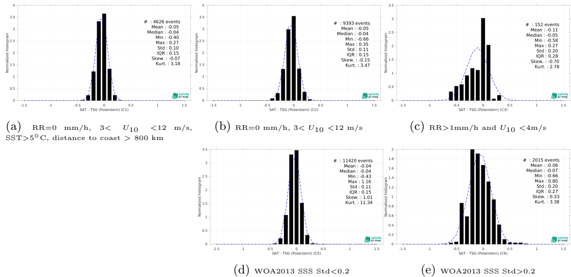
Figure 13: Normalized histogram of \Delta SSS (Aquarius SSS L4 OI v5 - Monthly (IPRC) - TSG (Polarstern)) for 5 different subdatasets corresponding to: RR=0 mm/h, 3 < U_{10} < 12 m/s, SST >5^\circ C, distance to coast > 800 km (a), RR=0 mm/h, 3 < U_{10} < 12 m/s (b), RR >1 mm/h and U_{10} < 4 m/s (c), WOA2013 SSS Std <0.2 (d), WOA2013 SSS Std >0.2 (e).
