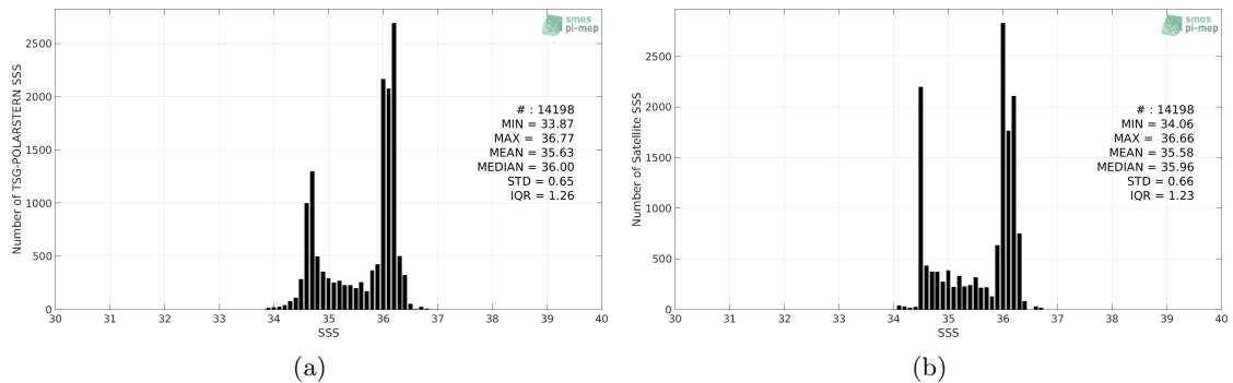
Figure 2: Histograms of SSS from TSG-POLARSTERN (a) and Aquarius-L4-IPRC-V5-MONTHLY (b) considering all match-up pairs per bins of 0.1 over the Equatorial Ocean 10N-10S Pi-MEP region and for the full satellite product period.
