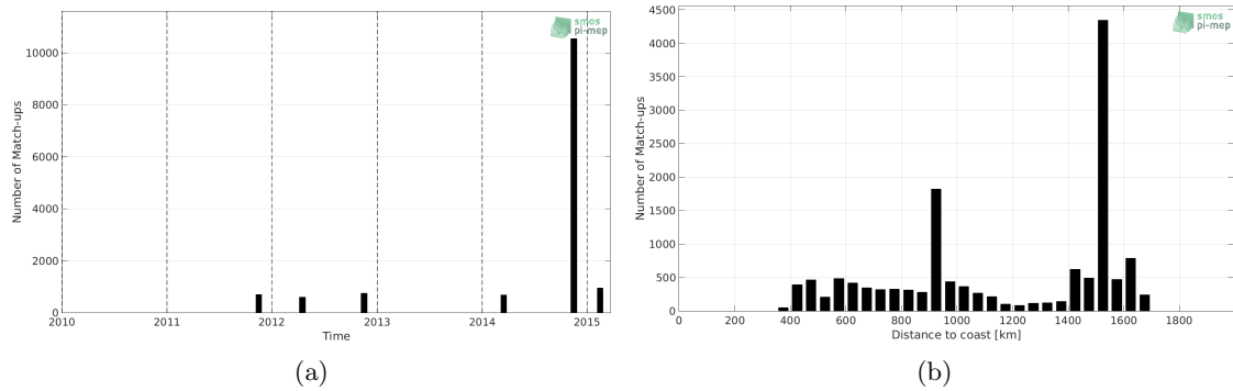
Figure 1: Number of match-ups between TSG-POLARSTERN and Aquarius-L4-IPRC-V5-MONTHLY SSS as a function of time (a) and as function of the distance to coast (b) over the Equatorial Ocean 10N-10S Pi-MEP region and for the full satellite product period.
