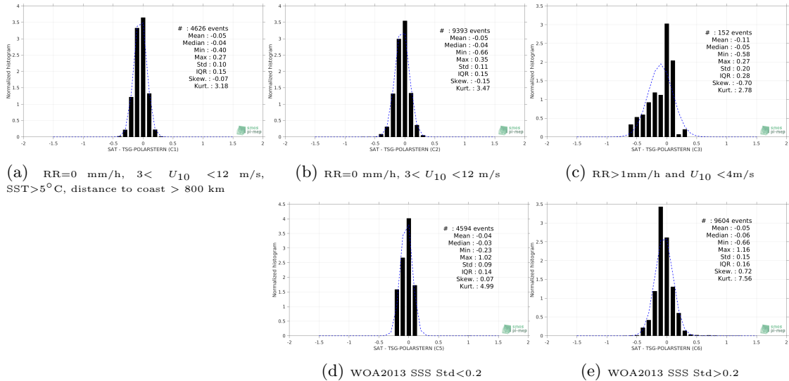
Figure 13: Normalized histogram of ΔSSS (Aquarius-L4-IPRC-V5-MONTHLY - TSG-POLARSTERN) for 5 different subdatasets corresponding to: RR=0 mm/h, 3 < U 10 < 12 m/s, SST>5°C, distance to coast > 800 km (a), RR=0 mm/h, 3 < U 10 < 12 m/s (b), RR>1mm/h and U 10 < 4m/s (c), WOA2013 SSS Std<0.2 (d), WOA2013 SSS Std>0.2 (e).
