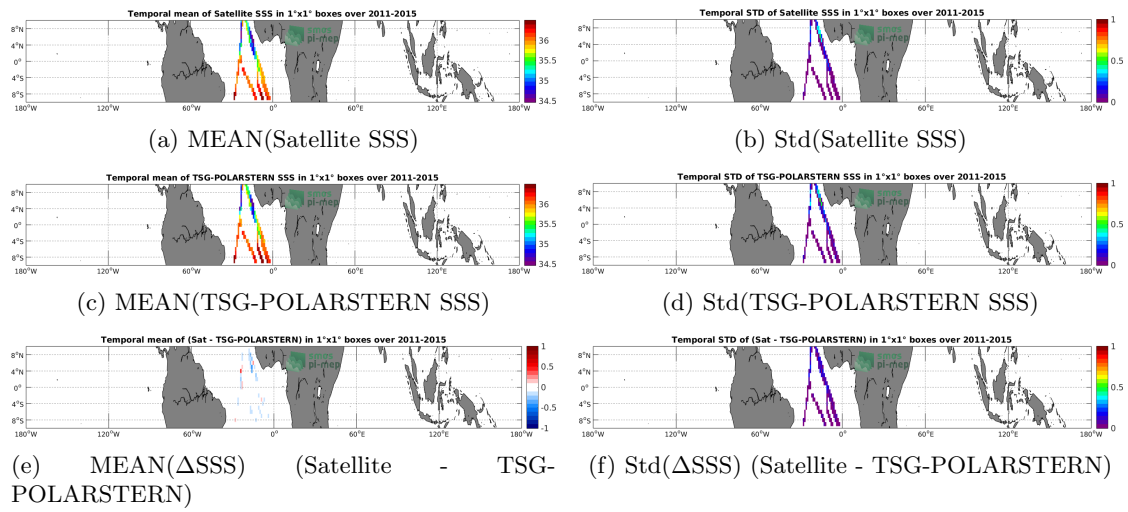
Figure 6: Temporal mean (left) and Std (right) of SSS from Aquarius-L4-IPRC-V5-MONTHLY (top), TSG-POLARSTERN (middle), and of \Delta SSS (Satellite - TSG-POLARSTERN). Only match-up pairs are used to generate these maps.
