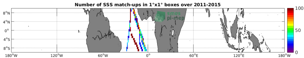
Figure 4: Number of SSS match-ups between TSG-POLARSTERN SSS and the Aquarius-L4-IPRC-V5-MONTHLY SSS product for the Equatorial Ocean 10N-10S Pi-MEP region over 1°x1° boxes and for the full satellite product period.
