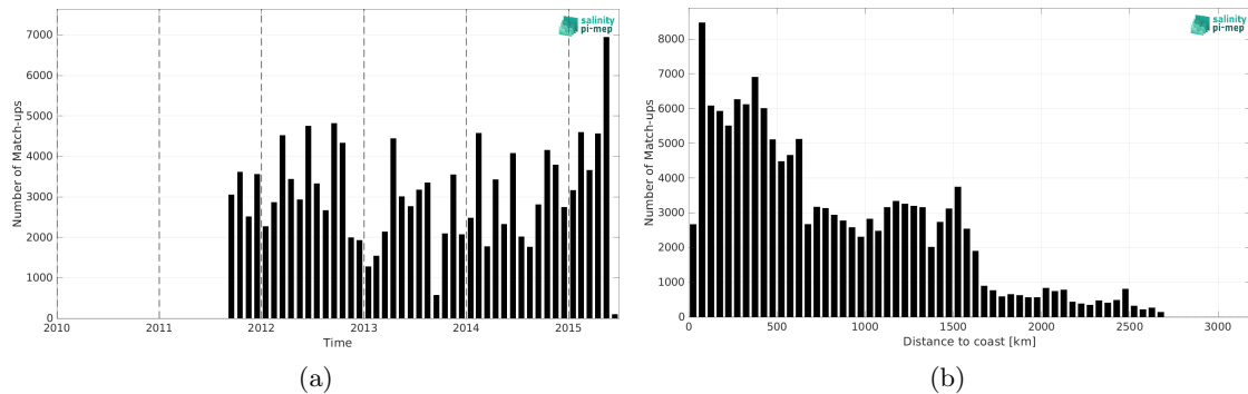
Figure 2: Number of match-ups between TSG (LEGOS-DM) and Aquarius SSS L4 OI v5 - Monthly (IPRC) SSS as a function of time (a) and as function of the distance to coast (b) over the Equatorial Ocean 10N-10S Pi-MEP region and for the full satellite product period.
