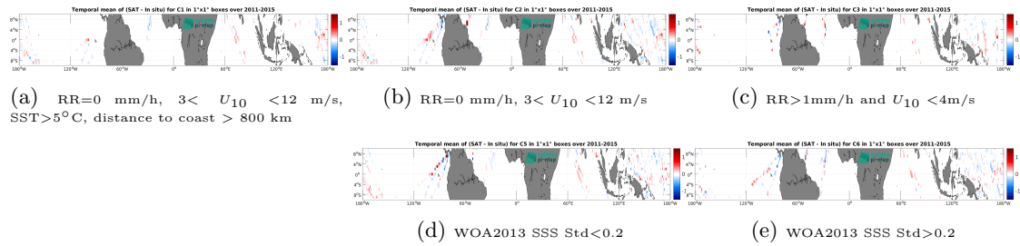
Figure 14: Temporal mean gridded over spatial boxes of size 1^\circ \times 1^\circ of \Delta SSS (Aquarius SSS L4 OI v5 - Monthly (IPRC) - TSG (LEGOS-DM)) for 5 different subdatasets corresponding to:RR=0 mm/h, 3 < U_{10} < 12 m/s, SST>5°C, distance to coast > 800 km (a), RR=0 mm/h, 3 < U_{10} < 12 m/s (b), RR>1mm/h and U_{10} < 4 m/s (c), WOA2013 SSS Std<0.2 (d), WOA2013 SSS Std>0.2 (e).
