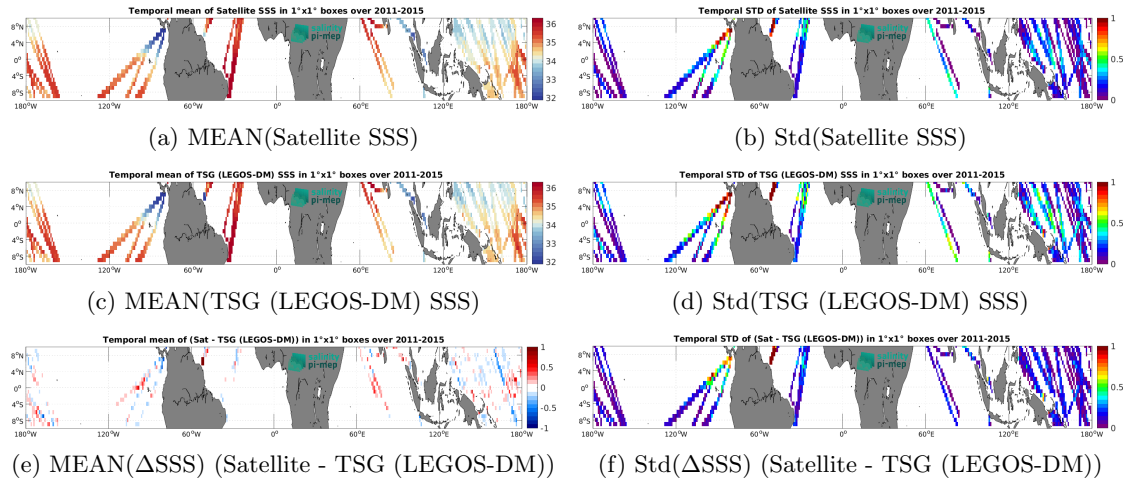
Figure 7: Temporal mean (left) and Std (right) of SSS from Aquarius SSS L4 OI v5 - Monthly (IPRC) (top), TSG (LEGOS-DM) (middle), and of \Delta SSS (Satellite - TSG (LEGOS-DM)). Only match-up pairs are used to generate these maps.
