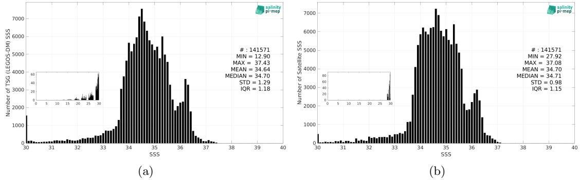
Figure 3: Histograms of SSS from TSG (LEGOS-DM) (a) and Aquarius SSS L4 OI v5 - Monthly (IPRC) (b) considering all match-up pairs per bins of 0.1 over the Equatorial Ocean 10N-10S Pi-MEP region and for the full satellite product period.
