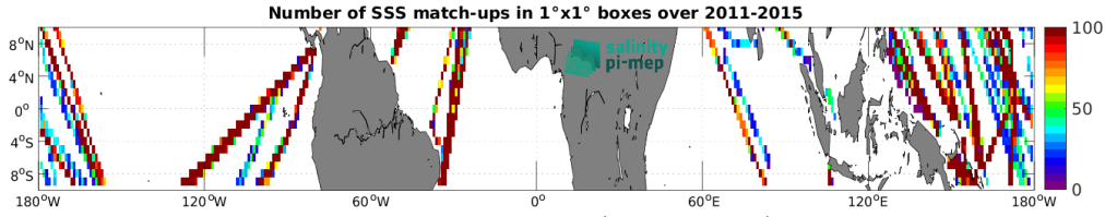
Figure 5: Number of SSS match-ups between TSG (LEGOS-DM) SSS and the Aquarius SSS L4 OI v5 - Monthly (IPRC) SSS product for the Equatorial Ocean 10N-10S Pi-MEP region over 1^\circ \times 1^\circ boxes and for the full satellite product period.
