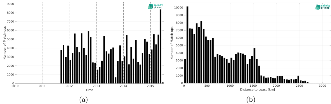
Figure 1: Number of match-ups between TSG (LEGOS-DM) and Aquarius SSS L4 OI v5 - Monthly (IPRC) SSS as a function of time (a) and as function of the distance to coast (b) over the Equatorial Ocean 10N-10S Pi-MEP region and for the full satellite product period.
