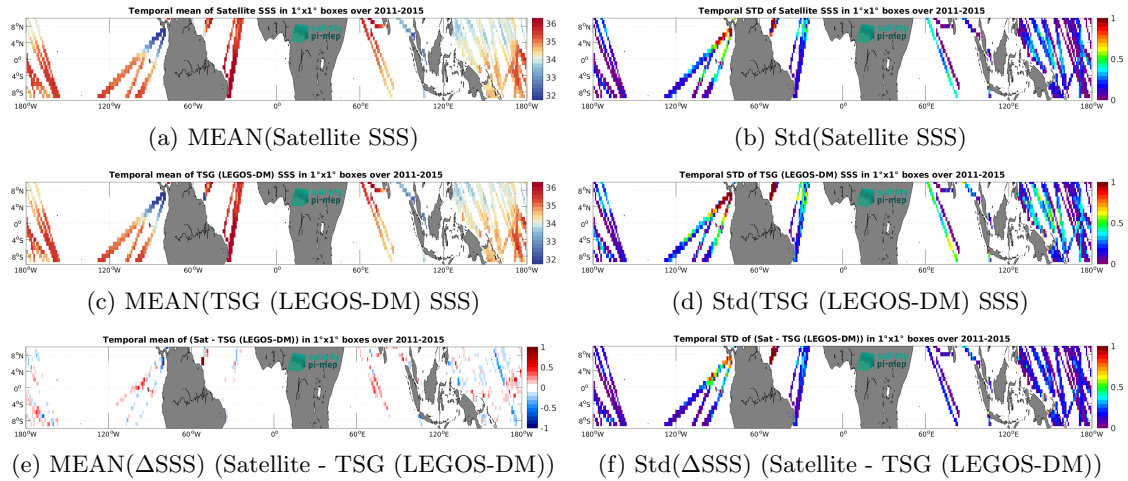
Figure 6: Temporal mean (left) and Std (right) of SSS from Aquarius SSS L4 OI v5 - Monthly (IPRC) (top), TSG (LEGOS-DM) ( in situ ) dataset (middle), and of \Delta SSS (Satellite - TSG (LEGOS-DM)). Only match-up pairs are used to generate these maps.
