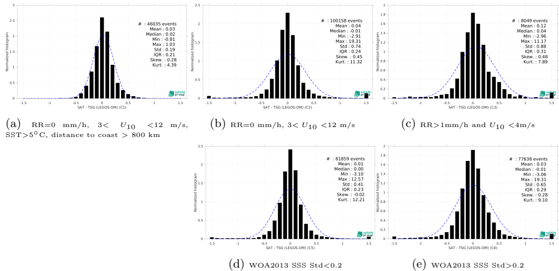
Figure 13: Normalized histogram of \Delta SSS (Aquarius SSS L4 OI v5 - Monthly (IPRC) - TSG (LEGOS-DM)) for 5 different subdatasets corresponding to: RR=0 mm/h, 3 < U_{10} < 12 m/s, SST > 5^\circ C , distance to coast > 800 km (a), RR=0 mm/h, 3 < U_{10} < 12 m/s (b), RR > 1 mm/h and U_{10} < 4 m/s (c), WOA2013 SSS Std < 0.2 (d), WOA2013 SSS Std > 0.2 (e).
