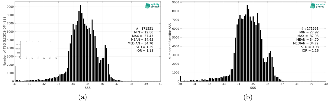
Figure 2: Histograms of SSS from TSG (LEGOS-DM) (a) and Aquarius SSS L4 OI v5 - Monthly (IPRC) (b) considering all match-up pairs per bins of 0.1 over the Equatorial Ocean 10N-10S Pi-MEP region and for the full satellite product period.
