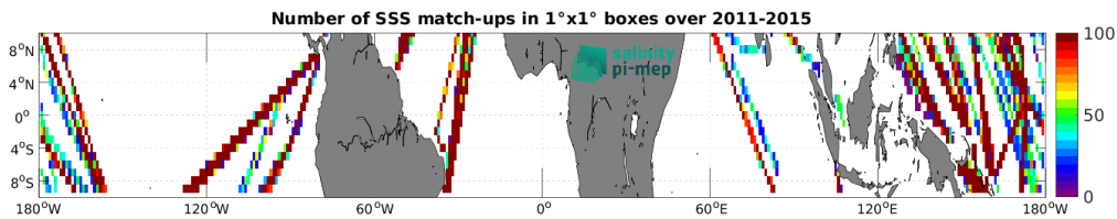
Figure 4: Number of SSS match-ups between TSG (LEGOS-DM) SSS and the Aquarius SSS L4 OI v5 - Monthly (IPRC) SSS product for the Equatorial Ocean 10N-10S Pi-MEP region over 1^\circ \times 1^\circ boxes and for the full satellite product period.
