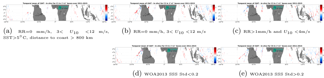
Figure 12: Temporal mean gridded over spatial boxes of size 1^\circ \times 1^\circ of \Delta SSS (Aquarius SSS L4 OI v5 - Monthly (IPRC) - TSG (LEGOS-DM)) for 5 different subdatasets corresponding to: RR=0 mm/h, 3 < U_{10} < 12 m/s, SST > 5^\circ C , distance to coast > 800 km (a), RR=0 mm/h, 3 < U_{10} < 12 m/s (b), RR > 1 mm/h and U_{10} < 4 m/s (c), WOA2013 SSS Std < 0.2 (d), WOA2013 SSS Std > 0.2 (e).
