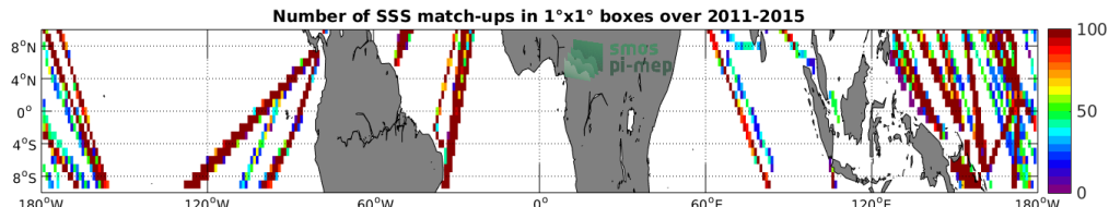
Figure 4: Number of SSS match-ups between TSG-LEGOS-DM SSS and the Aquarius-L4-IPRC-V5-MONTHLY SSS product for the Equatorial Ocean 10N-10S Pi-MEP region over 1°x1° boxes and for the full satellite product period.
