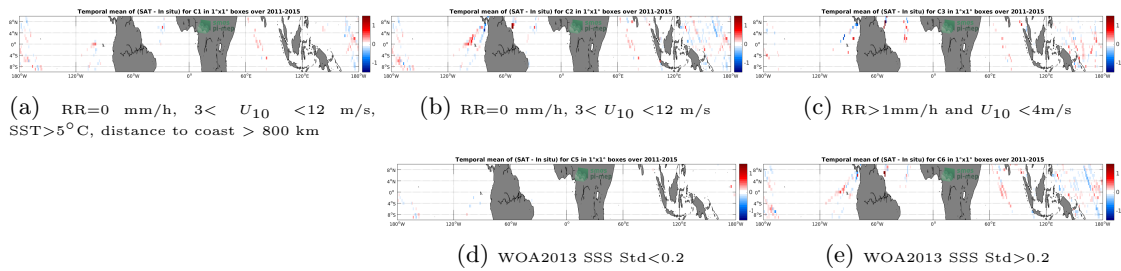
Figure 12: Temporal mean gridded over spatial boxes of size 1°x1° of ΔSSS (Aquarius-L4-IPRC-V5-MONTHLY - TSG-LEGOS-DM) for 5 different subdatasets corresponding to:RR=0 mm/h, 3 < U 10 < 12 m/s, SST > 5°C, distance to coast > 800 km (a), RR=0 mm/h, 3 < U 10 < 12 m/s (b), RR > 1mm/h and U 10 < 4m/s (c), WOA2013 SSS Std < 0.2 (d), WOA2013 SSS Std > 0.2 (e).
