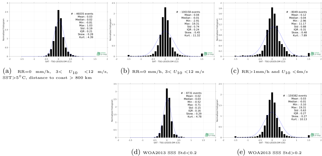
Figure 13: Normalized histogram of ΔSSS (Aquarius-L4-IPRC-V5-MONTHLY - TSG-LEGOS-DM) for 5 different subdatasets corresponding to: RR=0 mm/h, 3 < U 10 < 12 m/s, SST > 5°C, distance to coast > 800 km (a), RR=0 mm/h, 3 < U 10 < 12 m/s (b), RR > 1mm/h and U 10 < 4m/s (c), WOA2013 SSS Std < 0.2 (d), WOA2013 SSS Std > 0.2 (e).
