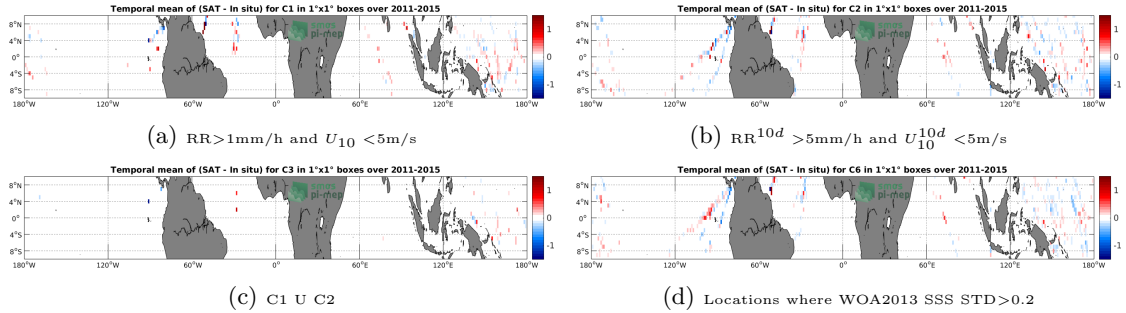
Figure 12: Temporal mean gridded over spatial boxes of size 1^\circ \times 1^\circ of \Delta SSS (Aquarius-L4-IPRC-V5-MONTHLY - TSG-LEGOS-DM) for 4 different subdatasets corresponding to: RR > 1\text{mm/h} and U_{10} < 5\text{m/s} (a), RR^{10d} > 5\text{mm/h} and U_{10}^{10d} < 5\text{m/s} (b), C1 U C2 (c), Locations where WOA2013 SSS STD > 0.2 (d).
