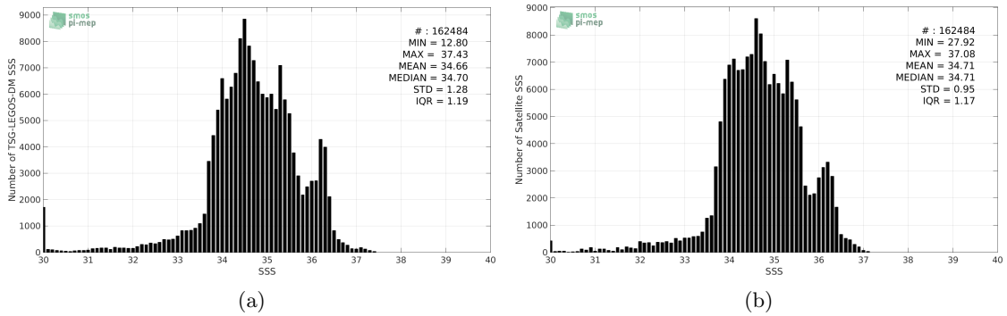
Figure 2: Histograms of SSS from TSG-LEGOS-DM (a) and Aquarius-L4-IPRC-V5-MONTHLY (b) considering all match-up pairs per bins of 0.1 over the Equatorial Ocean 10N-10S Pi-MEP region and for the full satellite product period.
