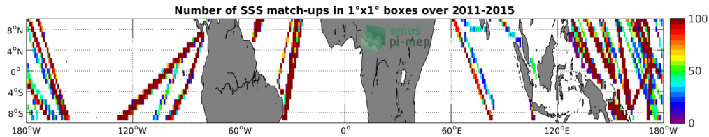
Figure 4: Number of SSS match-ups between TSG-LEGOS-DM SSS and the Aquarius-L4-IPRC-V5-MONTHLY SSS product for the Equatorial Ocean 10N-10S Pi-MEP region over 1^\circ \times 1^\circ boxes and for the full satellite product period.
