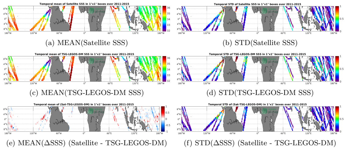
Figure 6: Temporal mean (left) and STD (right) of SSS from Aquarius-L4-IPRC-V5-MONTHLY (top), TSG-LEGOS-DM (middle), and of \Delta SSS (Satellite - TSG-LEGOS-DM). Only match-up pairs are used to generate these maps.
