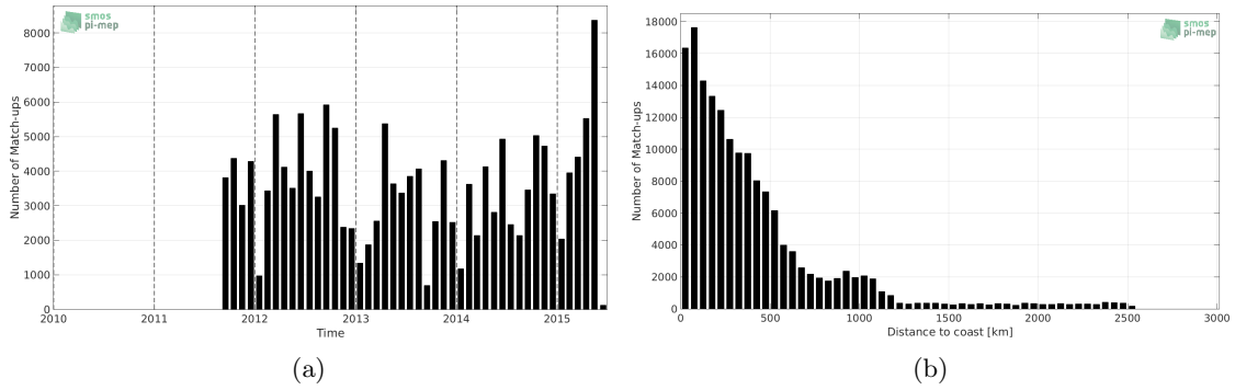
Figure 1: Number of match-ups between TSG-LEGOS-DM and Aquarius-L4-IPRC-V5-MONTHLY SSS as a function of time (a) and as function of the distance to coast (b) over the Equatorial Ocean 10N-10S Pi-MEP region and for the full satellite product period.
