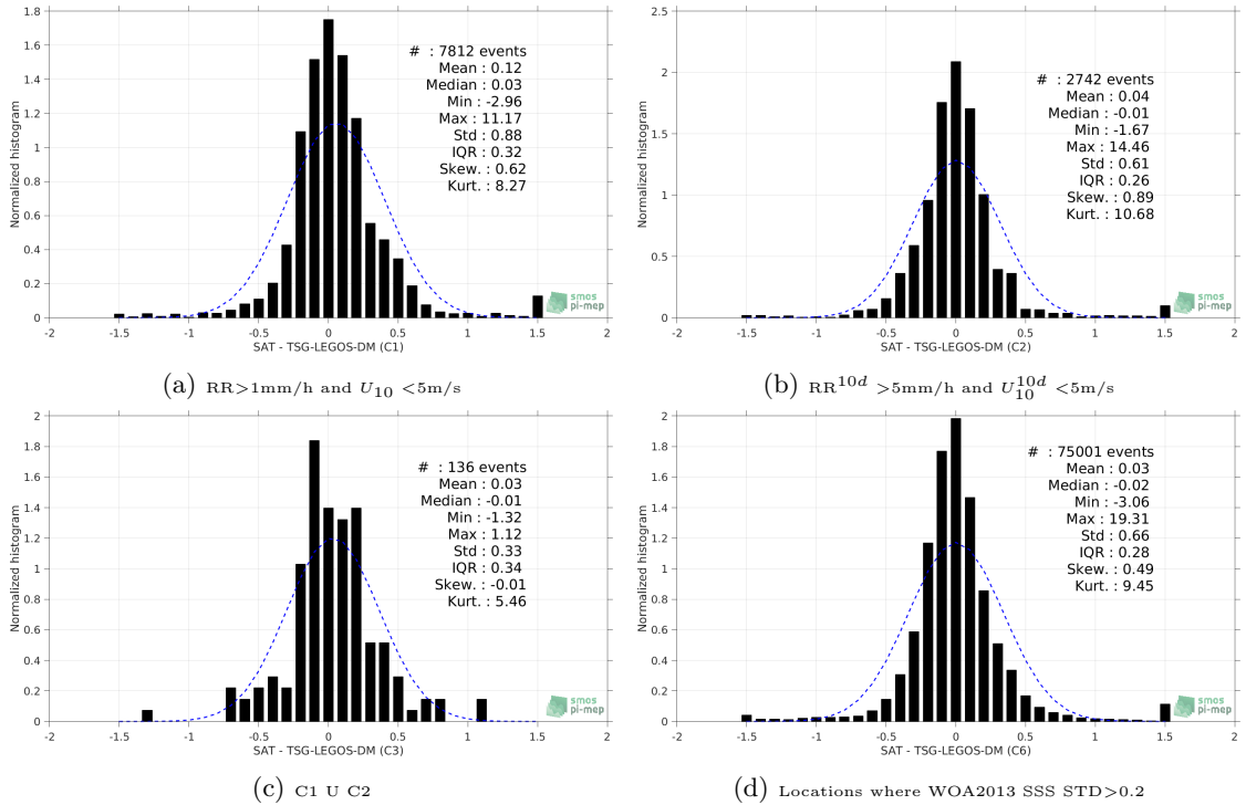
Figure 13: Normalized histogram of \Delta SSS (Aquarius-L4-IPRC-V5-MONTHLY - TSG-LEGOS-DM) for 6 different subdatasets corresponding to: RR > 1\text{mm/h} and U_{10} < 5\text{m/s} (a), RR^{10d} > 5\text{mm/h} and U_{10}^{10d} < 5\text{m/s} (b), C1 U C2 (c), Locations where WOA2013 SSS STD > 0.2 (d).
