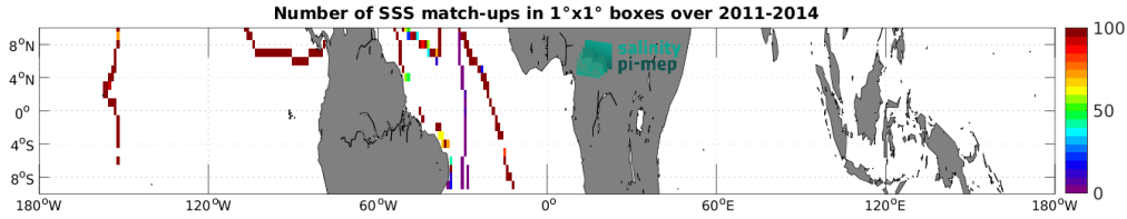
Figure 5: Number of SSS match-ups between TSG (GOSUD-Sailing-ship) SSS and the Aquarius SSS L4 OI v5 - Monthly (IPRC) SSS product for the Equatorial Ocean 10N-10S Pi-MEP region over 1^\circ \times 1^\circ boxes and for the full satellite product period.
