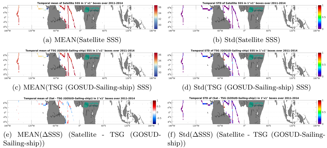
Figure 7: Temporal mean (left) and Std (right) of SSS from Aquarius SSS L4 OI v5 - Monthly (IPRC) (top), TSG (GOSUD-Sailing-ship) (middle), and of \Delta SSS (Satellite - TSG (GOSUD-Sailing-ship)). Only match-up pairs are used to generate these maps.
