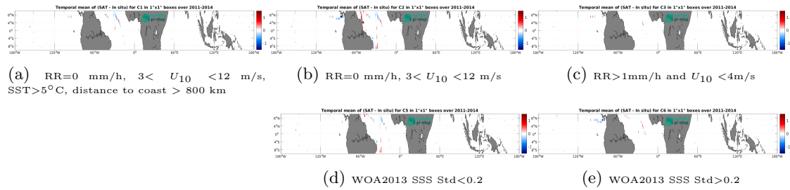
Figure 14: Temporal mean gridded over spatial boxes of size 1^\circ \times 1^\circ of \Delta SSS (Aquarius SSS L4 OI v5 - Monthly (IPRC) - TSG (GOSUD-Sailing-ship)) for 5 different subdatasets corresponding to: RR=0 mm/h, 3 < U_{10} < 12 m/s, SST>5°C, distance to coast > 800 km (a), RR=0 mm/h, 3 < U_{10} < 12 m/s (b), RR>1mm/h and U_{10} < 4 m/s (c), WOA2013 SSS Std<0.2 (d), WOA2013 SSS Std>0.2 (e).
