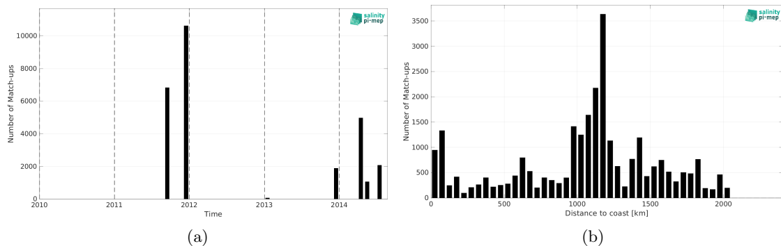
Figure 2: Number of match-ups between TSG (GOSUD-Sailing-ship) and Aquarius SSS L4 OI v5 - Monthly (IPRC) SSS as a function of time (a) and as function of the distance to coast (b) over the Equatorial Ocean 10N-10S Pi-MEP region and for the full satellite product period.
