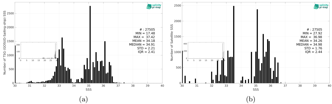
Figure 3: Histograms of SSS from TSG (GOSUD-Sailing-ship) (a) and Aquarius SSS L4 OI v5 - Monthly (IPRC) (b) considering all match-up pairs per bins of 0.1 over the Equatorial Ocean 10N-10S Pi-MEP region and for the full satellite product period.
