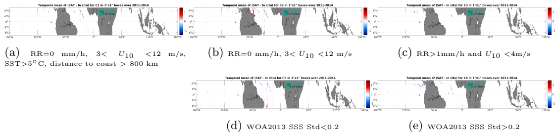
Figure 12: Temporal mean gridded over spatial boxes of size 1^\circ \times 1^\circ of \Delta SSS (Aquarius SSS L4 OI v5 - Monthly (IPRC) - TSG (GOSUD-Sailing-ship)) for 5 different subdatasets corresponding to: RR=0 mm/h, 3 < U_{10} < 12 m/s, SST>5°C, distance to coast > 800 km (a), RR=0 mm/h, 3 < U_{10} < 12 m/s (b), RR>1mm/h and U_{10} < 4 m/s (c), WOA2013 SSS Std<0.2 (d), WOA2013 SSS Std>0.2 (e).
