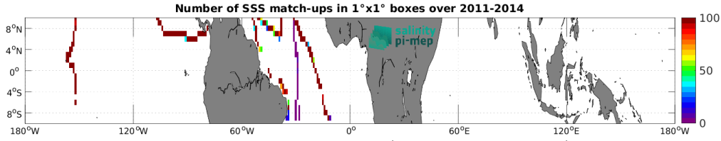
Figure 4: Number of SSS match-ups between TSG (GOSUD-Sailing-ship) SSS and the Aquarius SSS L4 OI v5 - Monthly (IPRC) SSS product for the Equatorial Ocean 10N-10S Pi-MEP region over 1^\circ \times 1^\circ boxes and for the full satellite product period.
