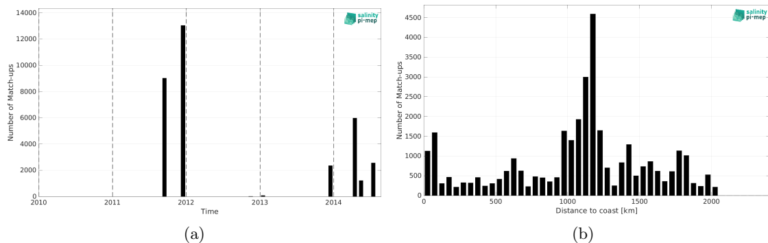
Figure 1: Number of match-ups between TSG (GOSUD-Sailing-ship) and Aquarius SSS L4 OI v5 - Monthly (IPRC) SSS as a function of time (a) and as function of the distance to coast (b) over the Equatorial Ocean 10N-10S Pi-MEP region and for the full satellite product period.
