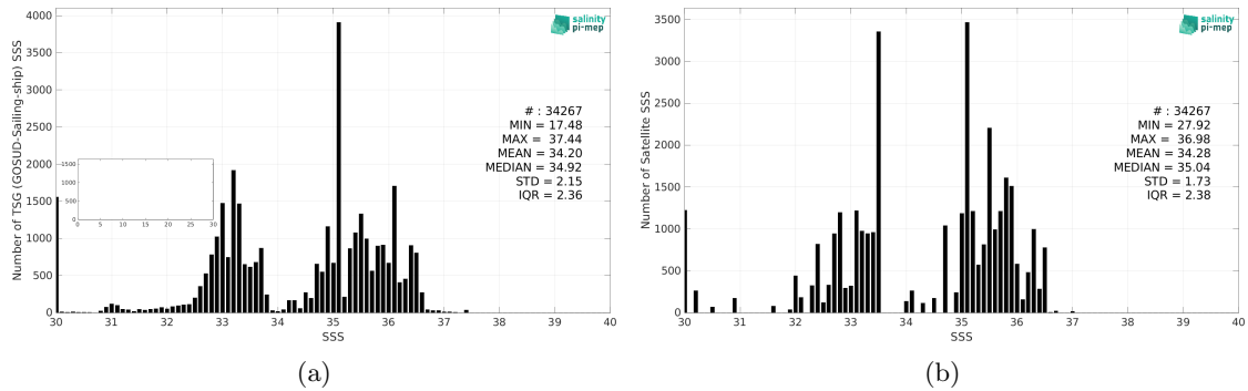
Figure 2: Histograms of SSS from TSG (GOSUD-Sailing-ship) (a) and Aquarius SSS L4 OI v5 - Monthly (IPRC) (b) considering all match-up pairs per bins of 0.1 over the Equatorial Ocean 10N-10S Pi-MEP region and for the full satellite product period.
