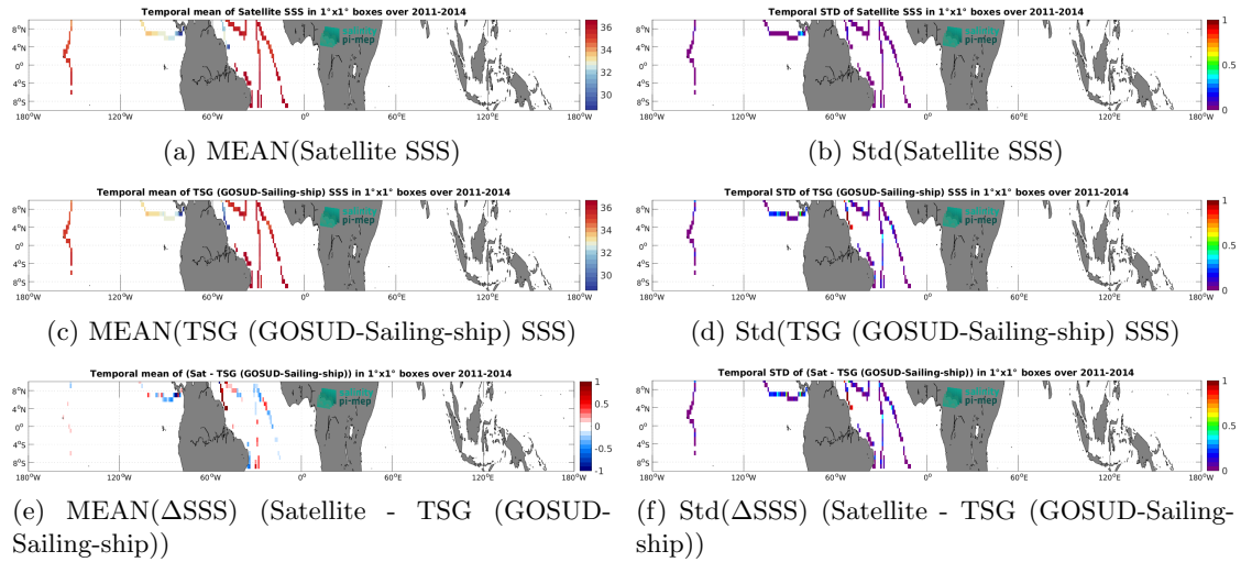
Figure 6: Temporal mean (left) and Std (right) of SSS from Aquarius SSS L4 OI v5 - Monthly (IPRC) (top), TSG (GOSUD-Sailing-ship) (middle), and of \Delta SSS (Satellite - TSG (GOSUD-Sailing-ship)). Only match-up pairs are used to generate these maps.
