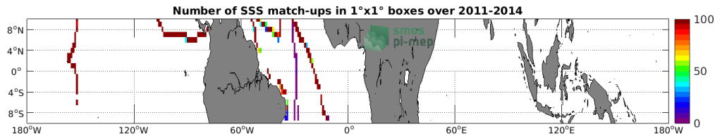
Figure 4: Number of SSS match-ups between TSG (GOSUD-Sailing-ship) SSS and the Aquarius SSS L4 OI v5 - Monthly (IPRC) SSS product for the Equatorial Ocean 10N-10S Pi-MEP region over 1°x1° boxes and for the full satellite product period.
