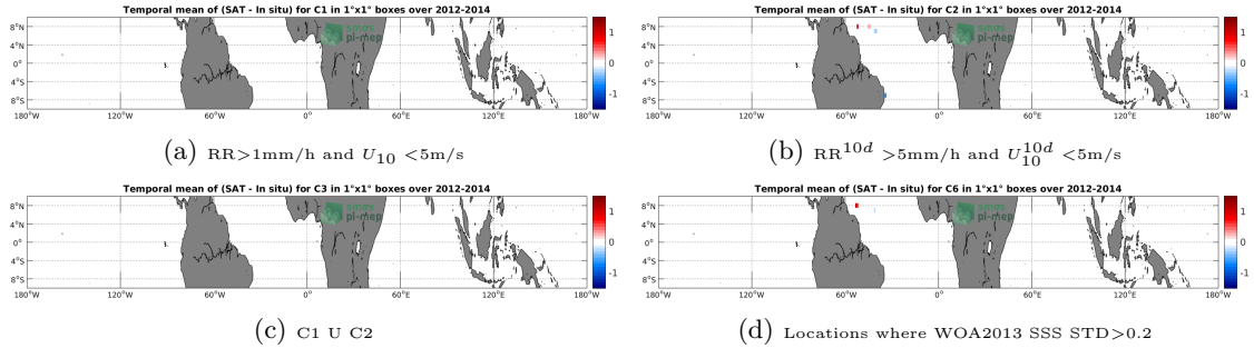
Figure 12: Temporal mean gridded over spatial boxes of size 1^\circ \times 1^\circ of \Delta SSS (Aquarius-L4-IPRC-V5-MONTHLY - TSG-GOSUD-Sailing-ship) for 4 different subdatasets corresponding to: RR > 1\text{mm/h} and U_{10} < 5\text{m/s} (a), RR^{10d} > 5\text{mm/h} and U_{10}^{10d} < 5\text{m/s} (b), C1 U C2 (c), Locations where WOA2013 SSS STD > 0.2 (d).
