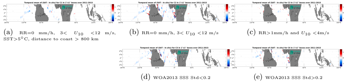
Figure 14: Temporal mean gridded over spatial boxes of size 1^\circ \times 1^\circ of \Delta SSS (Aquarius SSS L4 OI v5 - Monthly (IPRC) - TSG (GOSUD-Research-vessel)) for 5 different subdatasets corresponding to: RR=0 mm/h, 3 < U_{10} < 12 m/s, SST>5°C, distance to coast > 800 km (a), RR=0 mm/h, 3 < U_{10} < 12 m/s (b), RR>1mm/h and U_{10} < 4 m/s (c), WOA2013 SSS Std<0.2 (d), WOA2013 SSS Std>0.2 (e).
