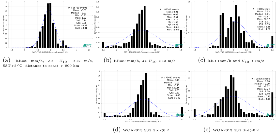
Figure 15: Normalized histogram of \Delta SSS (Aquarius SSS L4 OI v5 - Monthly (IPRC) - TSG (GOSUD-Research-vessel)) for 5 different subdatasets corresponding to: RR=0 mm/h, 3 < U_{10} < 12 m/s, SST>5°C, distance to coast > 800 km (a), RR=0 mm/h, 3 < U_{10} < 12 m/s (b), RR>1mm/h and U_{10} < 4 m/s (c), WOA2013 SSS Std<0.2 (d), WOA2013 SSS Std>0.2 (e).
