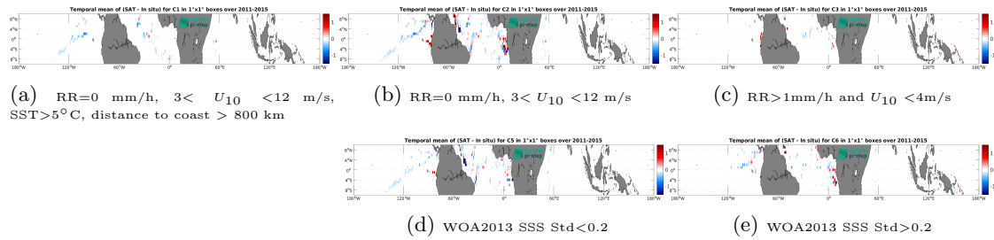
Figure 14: Temporal mean gridded over spatial boxes of size 1^\circ \times 1^\circ of \Delta SSS (Aquarius SSS L4 OI v5 - Monthly (IPRC) - TSG (GOSUD-Research-vessel)) for 5 different subdatasets corresponding to: RR=0 mm/h, 3 < U_{10} < 12 m/s, SST>5°C, distance to coast > 800 km (a), RR=0 mm/h, 3 < U_{10} < 12 m/s (b), RR>1mm/h and U_{10} < 4 m/s (c), WOA2013 SSS Std<0.2 (d), WOA2013 SSS Std>0.2 (e).
