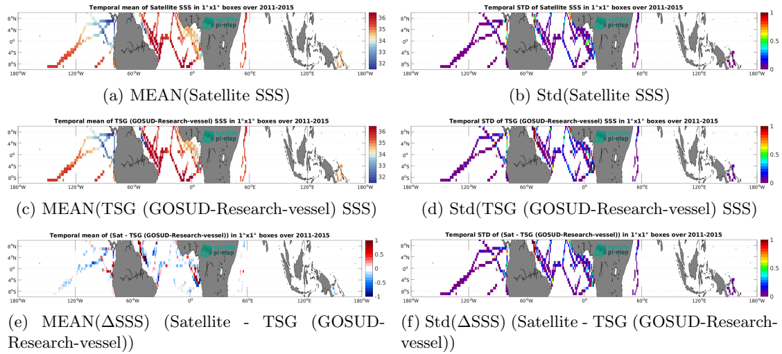
Figure 7: Temporal mean (left) and Std (right) of SSS from Aquarius SSS L4 OI v5 - Monthly (IPRC) (top), TSG (GOSUD-Research-vessel) (middle), and of \Delta SSS (Satellite - TSG (GOSUD-Research-vessel)). Only match-up pairs are used to generate these maps.
