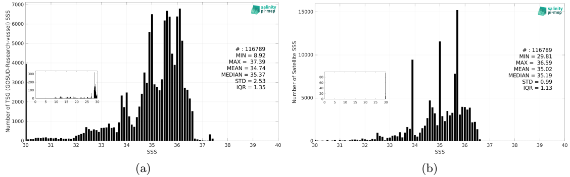
Figure 3: Histograms of SSS from TSG (GOSUD-Research-vessel) (a) and Aquarius SSS L4 OI v5 - Monthly (IPRC) (b) considering all match-up pairs per bins of 0.1 over the Equatorial Ocean 10N-10S Pi-MEP region and for the full satellite product period.
