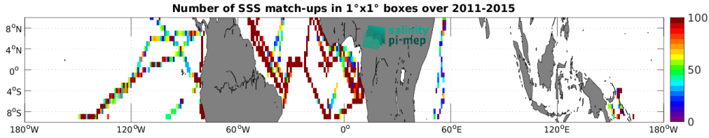
Figure 5: Number of SSS match-ups between TSG (GOSUD-Research-vessel) SSS and the Aquarius SSS L4 OI v5 - Monthly (IPRC) SSS product for the Equatorial Ocean 10N-10S Pi-MEP region over 1^\circ \times 1^\circ boxes and for the full satellite product period.
