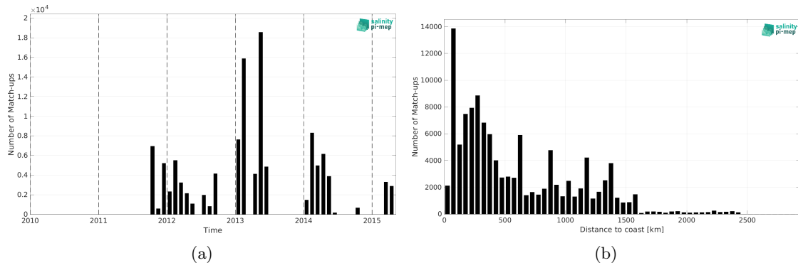
Figure 2: Number of match-ups between TSG (GOSUD-Research-vessel) and Aquarius SSS L4 OI v5 - Monthly (IPRC) SSS as a function of time (a) and as function of the distance to coast (b) over the Equatorial Ocean 10N-10S Pi-MEP region and for the full satellite product period.
