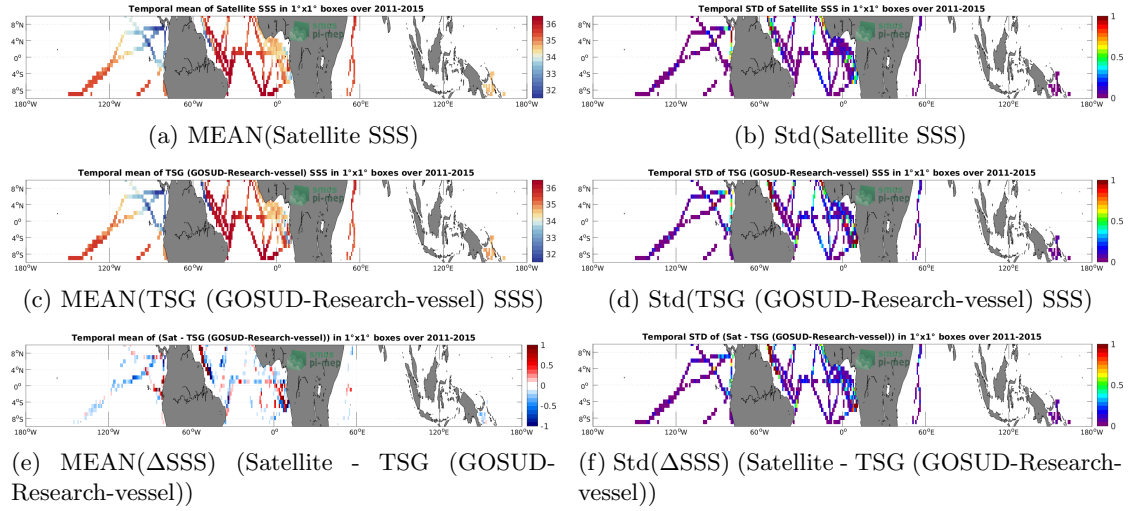
Figure 6: Temporal mean (left) and Std (right) of SSS from Aquarius SSS L4 OI v5 - Monthly (IPRC) (top), TSG (GOSUD-Research-vessel) (middle), and of \Delta SSS (Satellite - TSG (GOSUD-Research-vessel)). Only match-up pairs are used to generate these maps.
