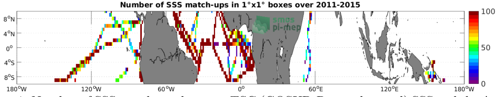
Figure 4: Number of SSS match-ups between TSG (GOSUD-Research-vessel) SSS and the Aquarius SSS L4 OI v5 - Monthly (IPRC) SSS product for the Equatorial Ocean 10N-10S Pi-MEP region over 1^\circ \times 1^\circ boxes and for the full satellite product period.
