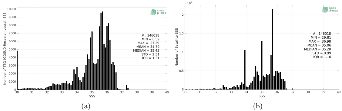
Figure 2: Histograms of SSS from TSG (GOSUD-Research-vessel) (a) and Aquarius SSS L4 OI v5 - Monthly (IPRC) (b) considering all match-up pairs per bins of 0.1 over the Equatorial Ocean 10N-10S Pi-MEP region and for the full satellite product period.
