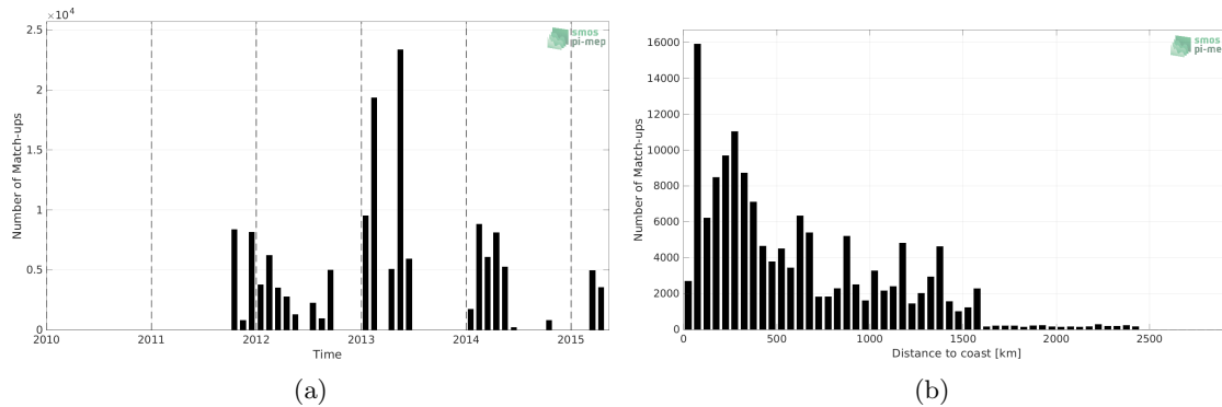
Figure 1: Number of match-ups between TSG (GOSUD-Research-vessel) and Aquarius SSS L4 OI v5 - Monthly (IPRC) SSS as a function of time (a) and as function of the distance to coast (b) over the Equatorial Ocean 10N-10S Pi-MEP region and for the full satellite product period.
