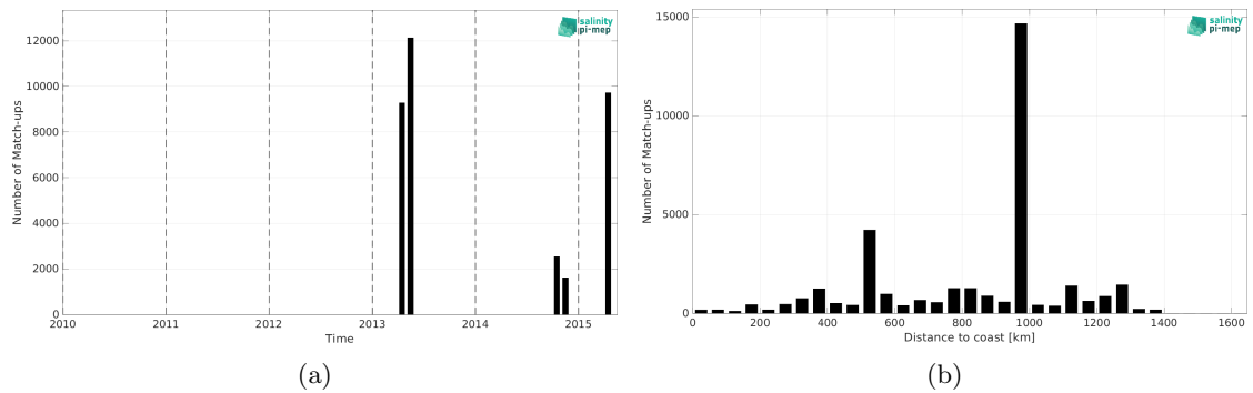
Figure 2: Number of match-ups between TSG (CSIC-UTM) and Aquarius SSS L4 OI v5 - Monthly (IPRC) SSS as a function of time (a) and as function of the distance to coast (b) over the Equatorial Ocean 10N-10S Pi-MEP region and for the full satellite product period.
