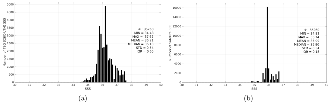
Figure 3: Histograms of SSS from TSG (CSIC-UTM) (a) and Aquarius SSS L4 OI v5 - Monthly (IPRC) (b) considering all match-up pairs per bins of 0.1 over the Equatorial Ocean 10N-10S Pi-MEP region and for the full satellite product period.
