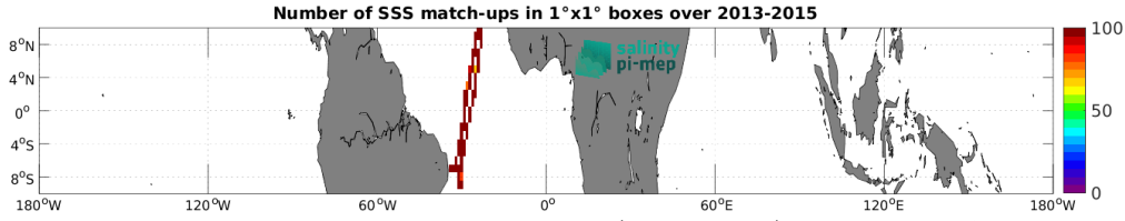
Figure 5: Number of SSS match-ups between TSG (CSIC-UTM) SSS and the Aquarius SSS L4 OI v5 - Monthly (IPRC) SSS product for the Equatorial Ocean 10N-10S Pi-MEP region over 1^\circ \times 1^\circ boxes and for the full satellite product period.
