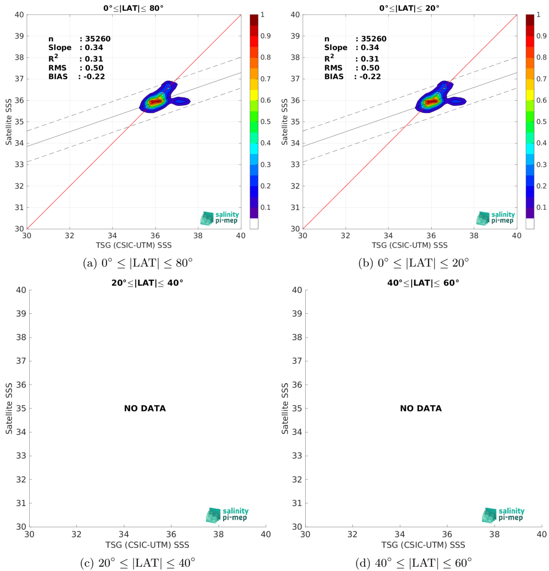
Figure 10: Contour maps of the concentration of Aquarius SSS L4 OI v5 - Monthly (IPRC) SSS (y-axis) versus TSG (CSIC-UTM) SSS (x-axis) at match-up pairs for different latitude bands. For each plot, the red line shows x=y . The black thin and dashed lines indicate a linear fit through the data cloud and the \pm 95\% confidence levels, respectively. The number match-up pairs n , the slope and R^2 coefficient of the linear fit, the root mean square (RMS) and the mean bias between satellite and in situ data are indicated for each latitude band in each plots.
