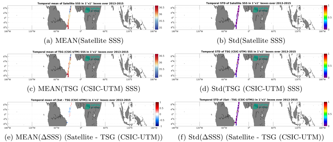
Figure 7: Temporal mean (left) and Std (right) of SSS from Aquarius SSS L4 OI v5 - Monthly (IPRC) (top), TSG (CSIC-UTM) (middle), and of \Delta SSS (Satellite - TSG (CSIC-UTM)). Only match-up pairs are used to generate these maps.
