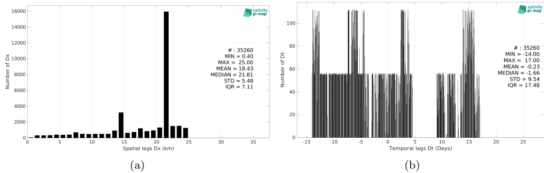
Figure 6: Histograms of the spatial (a) and temporal (b) lags between the location/time of the TSG (CSIC-UTM) measurement and the date of the corresponding Aquarius SSS L4 OI v5 - Monthly (IPRC) SSS pixel.
