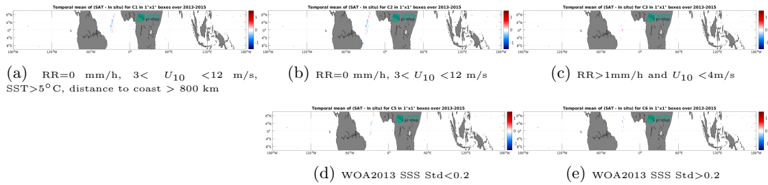
Figure 14: Temporal mean gridded over spatial boxes of size 1^\circ \times 1^\circ of \Delta SSS (Aquarius SSS L4 OI v5 - Monthly (IPRC) - TSG (CSIC-UTM)) for 5 different subdatasets corresponding to: RR=0 mm/h, 3 < U_{10} < 12 m/s, SST>5°C, distance to coast > 800 km (a), RR=0 mm/h, 3 < U_{10} < 12 m/s (b), RR>1mm/h and U_{10} < 4 m/s (c), WOA2013 SSS Std<0.2 (d), WOA2013 SSS Std>0.2 (e).
