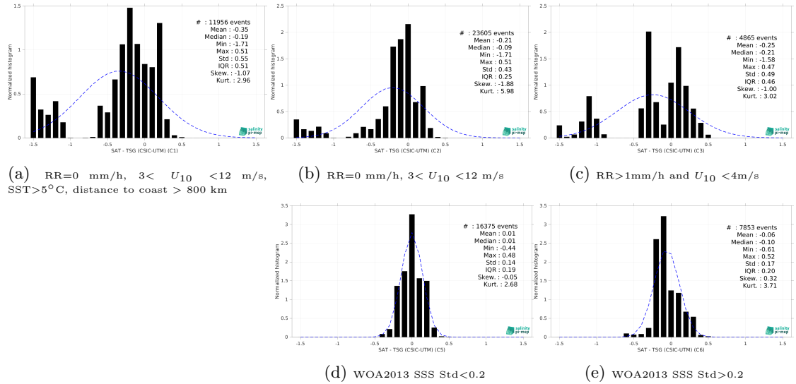
Figure 13: Normalized histogram of \Delta SSS (Aquarius SSS L4 OI v5 - Monthly (IPRC) - TSG (CSIC-UTM)) for 5 different subdatasets corresponding to: RR=0 mm/h, 3 < U_{10} < 12 m/s, SST >5^\circ C, distance to coast > 800 km (a), RR=0 mm/h, 3 < U_{10} < 12 m/s (b), RR >1 mm/h and U_{10} < 4 m/s (c), WOA2013 SSS Std <0.2 (d), WOA2013 SSS Std >0.2 (e).
