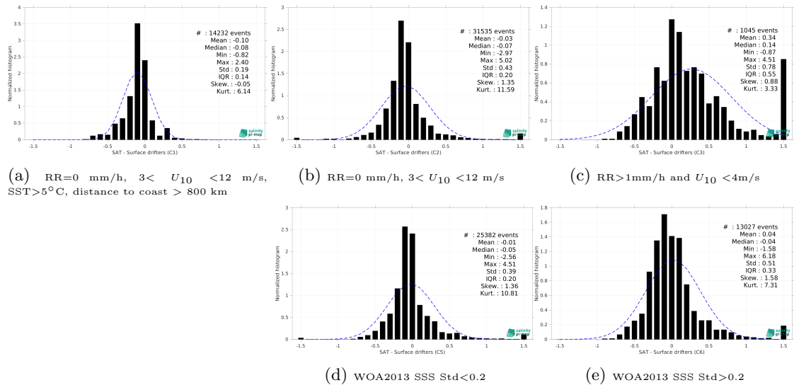
Figure 14: Normalized histogram of \Delta SSS (Aquarius SSS L4 OI v5 - Monthly (IPRC) - Surface drifters) for 5 different subdatasets corresponding to: RR=0 mm/h, 3 < U_{10} < 12 m/s, SST >5^\circ C, distance to coast > 800 km (a), RR=0 mm/h, 3 < U_{10} < 12 m/s (b), RR >1 mm/h and U_{10} < 4 m/s (c), WOA2013 SSS Std <0.2 (d), WOA2013 SSS Std >0.2 (e).
