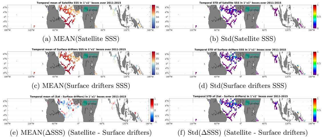
Figure 6: Temporal mean (left) and Std (right) of SSS from Aquarius SSS L4 OI v5 - Monthly (IPRC) (top), Surface drifters (middle), and of \Delta SSS (Satellite - Surface drifters). Only match-up pairs are used to generate these maps.
