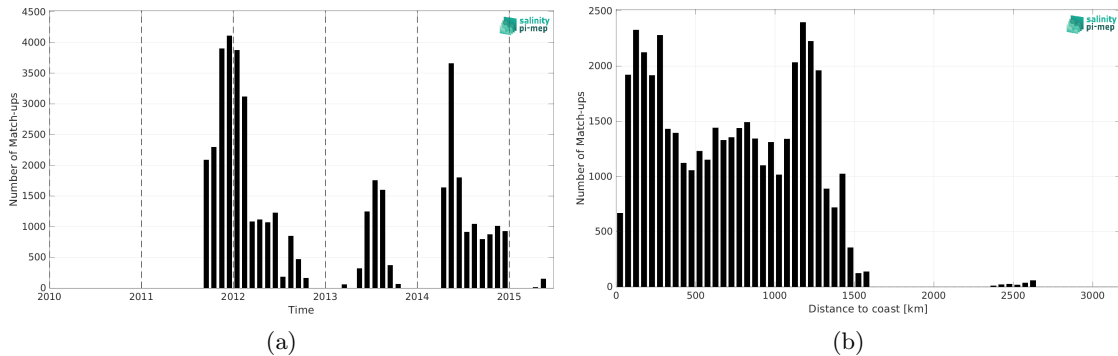
Figure 2: Number of match-ups between Surface drifters and Aquarius SSS L4 OI v5 - Monthly (IPRC) SSS as a function of time (a) and as function of the distance to coast (b) over the Equatorial Ocean 10N-10S Pi-MEP region and for the full satellite product period.
