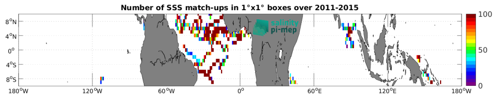
Figure 4: Number of SSS match-ups between Surface drifters SSS and the Aquarius SSS L4 OI v5 - Monthly (IPRC) SSS product for the Equatorial Ocean 10N-10S Pi-MEP region over 1^\circ \times 1^\circ boxes and for the full satellite product period.
