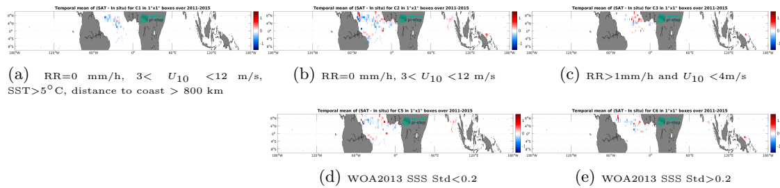
Figure 13: Temporal mean gridded over spatial boxes of size 1^\circ \times 1^\circ of \Delta SSS (Aquarius SSS L4 OI v5 - Monthly (IPRC) - Surface drifters) for 5 different subdatasets corresponding to: RR=0 mm/h, 3 < U_{10} < 12 m/s, SST > 5^\circ\text{C} , distance to coast > 800 km (a), RR=0 mm/h, 3 < U_{10} < 12 m/s (b), RR > 1 mm/h and U_{10} < 4 m/s (c), WOA2013 SSS Std < 0.2 (d), WOA2013 SSS Std > 0.2 (e).
