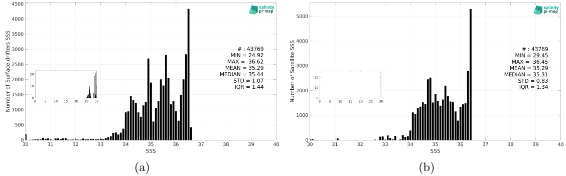
Figure 3: Histograms of SSS from Surface drifters (a) and Aquarius SSS L4 OI v5 - Monthly (IPRC) (b) considering all match-up pairs per bins of 0.1 over the Equatorial Ocean 10N-10S Pi-MEP region and for the full satellite product period.
