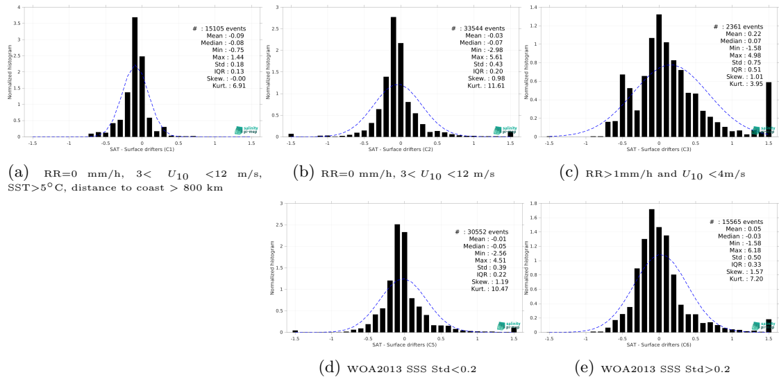
Figure 12: Normalized histogram of \Delta SSS (Aquarius SSS L4 OI v5 - Monthly (IPRC) - Surface drifters) for 5 different subdatasets corresponding to: RR=0 mm/h, 3 < U_{10} < 12 m/s, SST >5^\circ C, distance to coast > 800 km (a), RR=0 mm/h, 3 < U_{10} < 12 m/s (b), RR >1 mm/h and U_{10} < 4 m/s (c), WOA2013 SSS Std <0.2 (d), WOA2013 SSS Std >0.2 (e).
