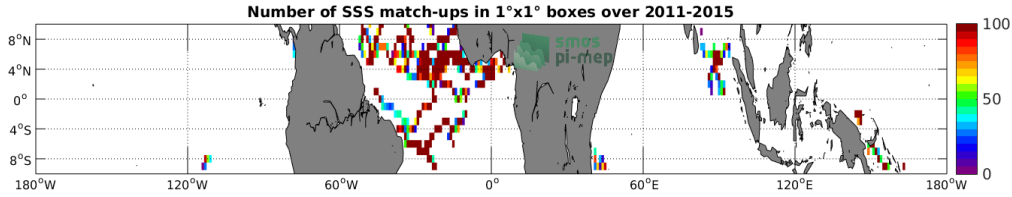
Figure 3: Number of SSS match-ups between Surface drifters SSS and the Aquarius-L4-IPRC-V5-MONTHLY SSS product for the Equatorial Ocean 10N-10S Pi-MEP region over 1^\circ \times 1^\circ boxes and for the full satellite product period.
