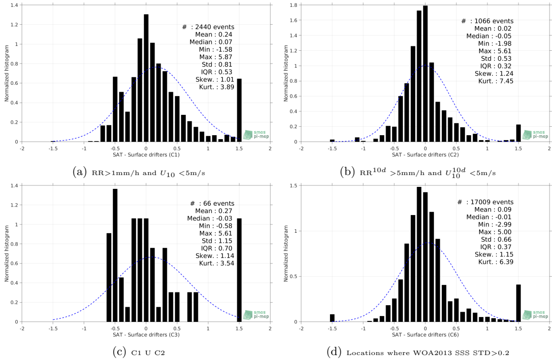
Figure 12: Normalized histogram of \Delta SSS (Aquarius-L4-IPRC-V5-MONTHLY - Surface drifters) for 6 different subdatasets corresponding to: RR >1 mm/h and U_{10} < 5 m/s (a), RR ^{10d} > 5 mm/h and U_{10}^{10d} < 5 m/s (b), C1 U C2 (c), Locations where WOA2013 SSS STD >0.2 (d).
