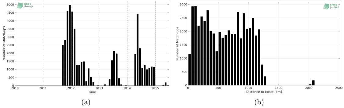
Figure 1: Number of match-ups between Surface drifters and Aquarius-L4-IPRC-V5-MONTHLY SSS as a function of time (a) and as function of the distance to coast (b) over the Equatorial Ocean 10N-10S Pi-MEP region and for the full satellite product period.
