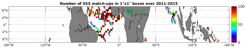
Figure 3: Number of SSS match-ups between Surface drifters SSS and the Aquarius-L4-IPRC-V5-MONTHLY SSS product for the Equatorial Ocean 10N-10S Pi-MEP region over 1^\circ \times 1^\circ boxes and for the full satellite product period.
