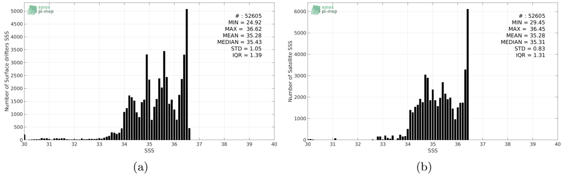
Figure 2: Histograms of SSS from Surface drifters (a) and Aquarius-L4-IPRC-V5-MONTHLY (b) considering all match-up pairs per bins of 0.1 over the Equatorial Ocean 10N-10S Pi-MEP region and for the full satellite product period.
