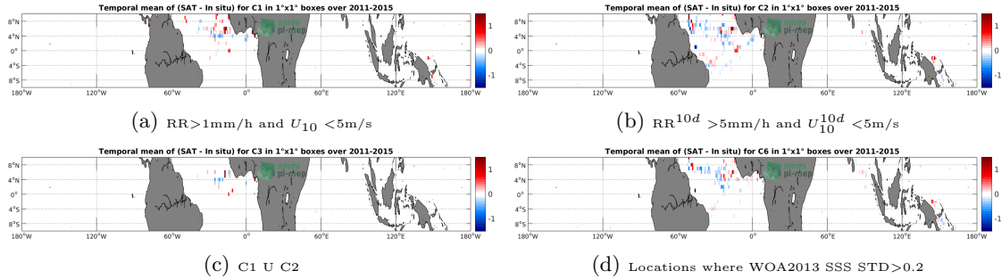
Figure 11: Temporal mean gridded over spatial boxes of size 1^\circ \times 1^\circ of \Delta SSS (Aquarius-L4-IPRC-V5-MONTHLY - Surface drifters) for 4 different subdatasets corresponding to: RR >1 mm/h and U_{10} < 5 m/s (a), RR ^{10d} > 5 mm/h and U_{10}^{10d} < 5 m/s (b), C1 U C2 (c), Locations where WOA2013 SSS STD >0.2 (d).
