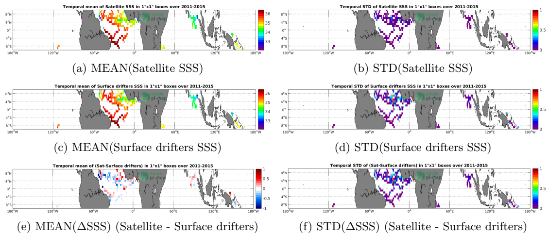
Figure 5: Temporal mean (left) and STD (right) of SSS from Aquarius-L4-IPRC-V5-MONTHLY (top), Surface drifters (middle), and of \Delta SSS (Satellite - Surface drifters). Only match-up pairs are used to generate these maps.
