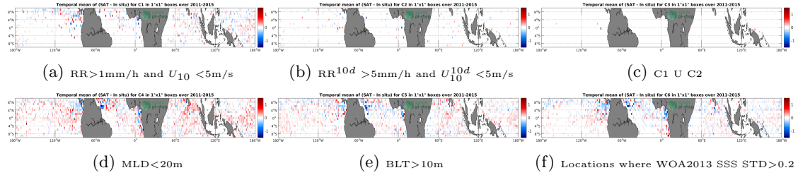
Figure 12: Temporal mean gridded over spatial boxes of size 1^\circ \times 1^\circ of \Delta SSS (Aquarius-L4-IPRC-V5-MONTHLY - Argo) for 6 different subdatasets corresponding to: RR > 1\text{mm/h} and U_{10} < 5\text{m/s} (a), RR^{10d} > 5\text{mm/h} and U_{10}^{10d} < 5\text{m/s} (b), C1 U C2 (c), MLD < 20\text{m} (d), BLT > 10\text{m} (e), Locations where WOA2013 SSS STD > 0.2 (f).
