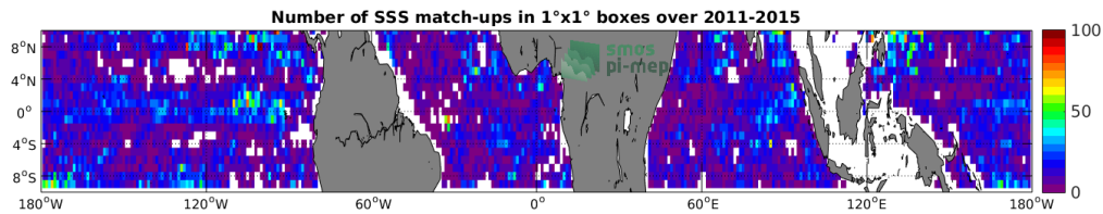
Figure 4: Number of SSS match-ups between Argo SSS and the Aquarius-L4-IPRC-V5-MONTHLY SSS product for the Equatorial Ocean 10N-10S Pi-MEP region over 1^\circ \times 1^\circ boxes and for the full satellite product period.
