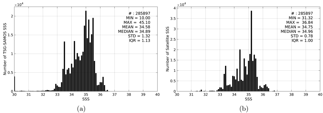
Figure 2: Histograms of SSS from TSG-SAMOS (a) and Aquarius-L4-IPRC-V4-WEEKLY (b) considering all match-up pairs per bins of 0.1 over the Equatorial Ocean 10N-10S Pi-MEP region and for the full satellite product period.
