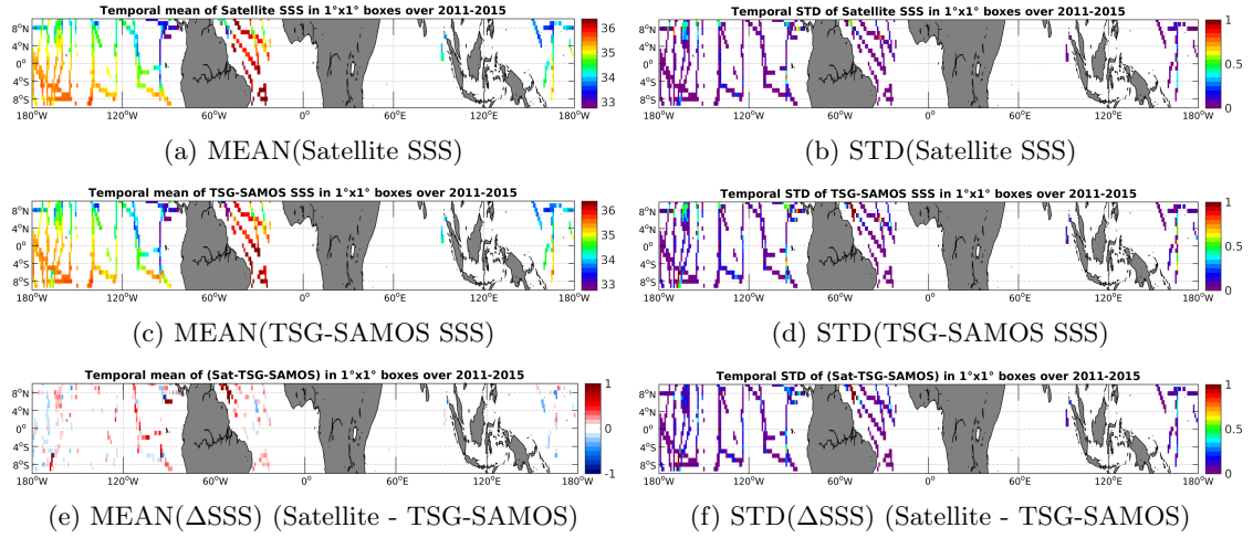
Figure 6: Temporal mean (left) and STD (right) of SSS from Aquarius-L4-IPRC-V4-WEEKLY (top), TSG-SAMOS (middle), and of \Delta SSS (Satellite - TSG-SAMOS). Only match-up pairs are used to generate these maps.
