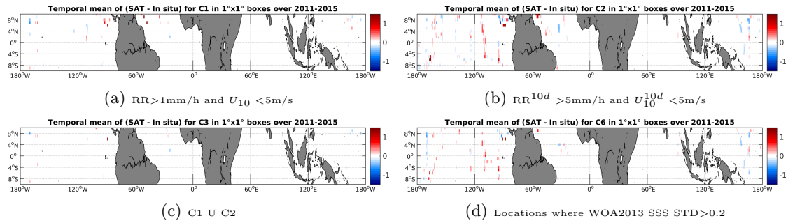
Figure 12: Temporal mean gridded over spatial boxes of size 1^\circ \times 1^\circ of \Delta SSS (Aquarius-L4-IPRC-V4-WEEKLY - TSG-SAMOS) for 4 different subdatasets corresponding to:RR >1 mm/h and U_{10} < 5 m/s (a), RR 10d > 5 mm/h and U_{10}^{10d} < 5 m/s (b), C1 U C2 (c),Locations where WOA2013 SSS STD >0.2 (d).
