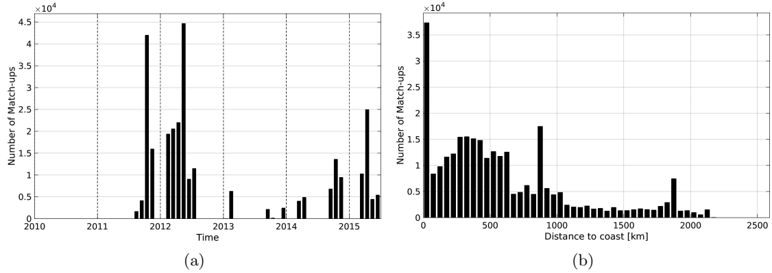
Figure 1: Number of match-ups between TSG-SAMOS and Aquarius-L4-IPRC-V4-WEEKLY SSS as a function of time (a) and as function of the distance to coast (b) over the Equatorial Ocean 10N-10S Pi-MEP region and for the full satellite product period.
