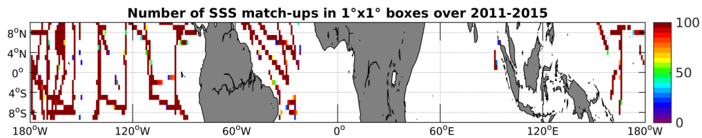
Figure 4: Number of SSS match-ups between TSG-SAMOS SSS and the Aquarius-L4-IPRC-V4-WEEKLY SSS product for the Equatorial Ocean 10N-10S Pi-MEP region over 1^\circ \times 1^\circ boxes and for the full satellite product period.
