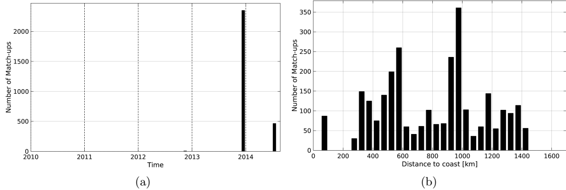
Figure 1: Number of match-ups between TSG-GOSUD-Sailing-ship and Aquarius-L4-IPRC-V4-WEEKLY SSS as a function of time (a) and as function of the distance to coast (b) over the Equatorial Ocean 10N-10S Pi-MEP region and for the full satellite product period.
