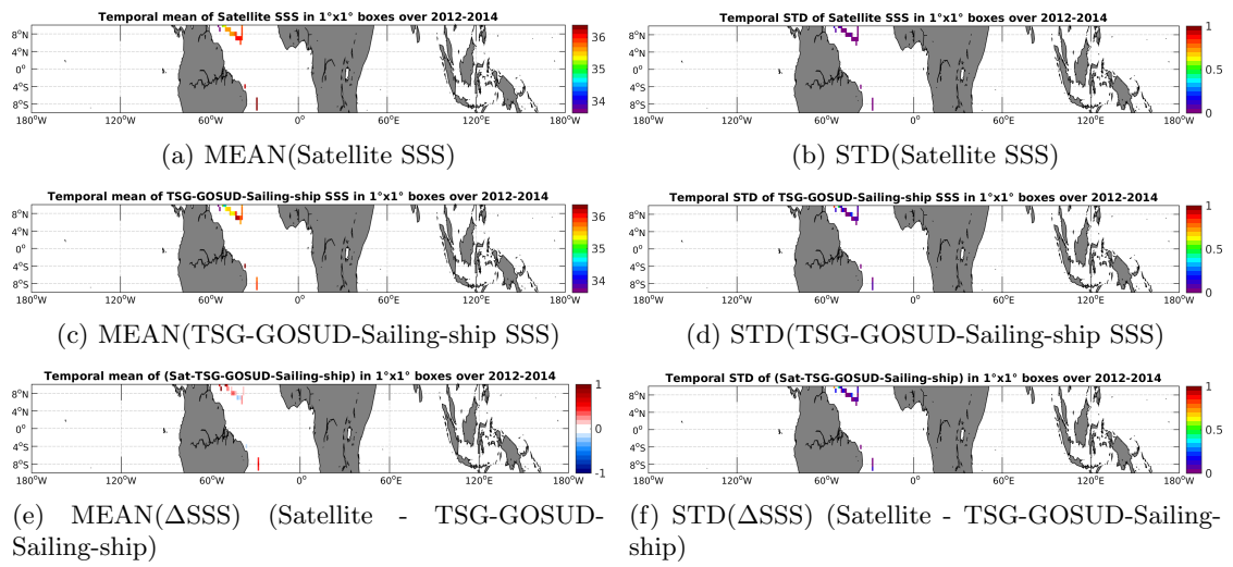
Figure 6: Temporal mean (left) and STD (right) of SSS from Aquarius-L4-IPRC-V4-WEEKLY (top), TSG-GOSUD-Sailing-ship (middle), and of \Delta SSS (Satellite - TSG-GOSUD-Sailing-ship). Only match-up pairs are used to generate these maps.
