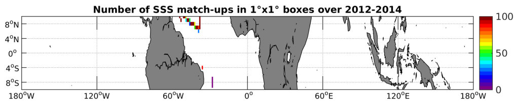
Figure 4: Number of SSS match-ups between TSG-GOSUD-Sailing-ship SSS and the Aquarius-L4-IPRC-V4-WEEKLY SSS product for the Equatorial Ocean 10N-10S Pi-MEP region over 1^\circ \times 1^\circ boxes and for the full satellite product period.
