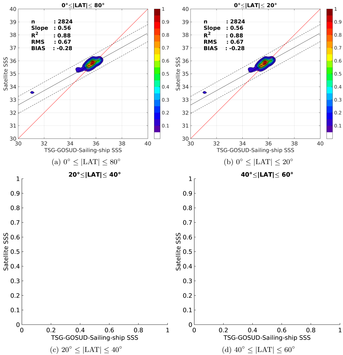
Figure 9: Contour maps of the concentration of Aquarius-L4-IPRC-V4-WEEKLY SSS (y-axis) versus TSG-GOSUD-Sailing-ship SSS (x-axis) at match-up pairs for different latitude bands. For each plot, the red line shows x=y . The black thin and dashed lines indicate a linear fit through the data cloud and the \pm 95\% confidence levels, respectively. The number match-up pairs n , the slope and R^2 coefficient of the linear fit, the root mean square (RMS) and the mean bias between satellite and in situ data are indicated for each latitude band in each plots.
