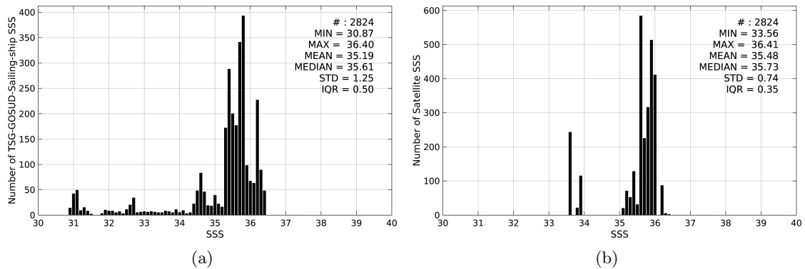
Figure 2: Histograms of SSS from TSG-GOSUD-Sailing-ship (a) and Aquarius-L4-IPRC-V4-WEEKLY (b) considering all match-up pairs per bins of 0.1 over the Equatorial Ocean 10N-10S Pi-MEP region and for the full satellite product period.
