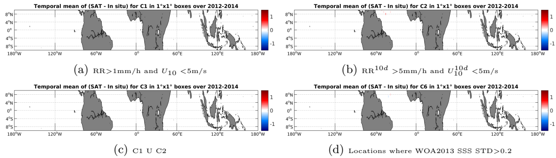
Figure 12: Temporal mean gridded over spatial boxes of size 1^\circ \times 1^\circ of \Delta SSS (Aquarius-L4-IPRC-V4-WEEKLY - TSG-GOSUD-Sailing-ship) for 4 different subdatasets corresponding to: RR > 1\text{mm/h} and U_{10} < 5\text{m/s} (a), RR^{10d} > 5\text{mm/h} and U_{10}^{10d} < 5\text{m/s} (b), C1 U C2 (c), Locations where WOA2013 SSS STD > 0.2 (d).
