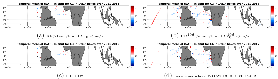
Figure 12: Temporal mean gridded over spatial boxes of size 1^\circ \times 1^\circ of \Delta SSS (Aquarius-L4-IPRC-V4-WEEKLY - TSG-GOSUD-Research-vessel) for 4 different subdatasets corresponding to:RR > 1 mm/h and U_{10} < 5 m/s (a), RR^{10d} > 5 mm/h and U_{10}^{10d} < 5 m/s (b), C1 U C2 (c),Locations where WOA2013 SSS STD > 0.2 (d).
