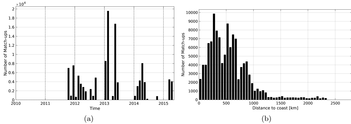
Figure 1: Number of match-ups between TSG-GOSUD-Research-vessel and Aquarius-L4-IPRC-V4-WEEKLY SSS as a function of time (a) and as function of the distance to coast (b) over the Equatorial Ocean 10N-10S Pi-MEP region and for the full satellite product period.
