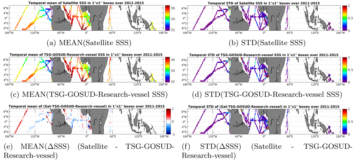
Figure 6: Temporal mean (left) and STD (right) of SSS from Aquarius-L4-IPRC-V4-WEEKLY (top), TSG-GOSUD-Research-vessel (middle), and of \Delta SSS (Satellite - TSG-GOSUD-Research-vessel). Only match-up pairs are used to generate these maps.
