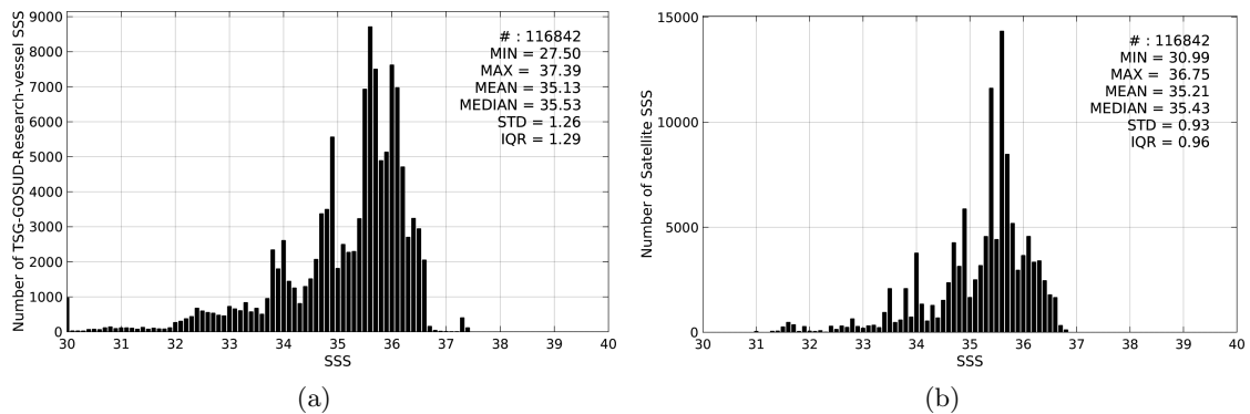
Figure 2: Histograms of SSS from TSG-GOSUD-Research-vessel (a) and Aquarius-L4-IPRC-V4-WEEKLY (b) considering all match-up pairs per bins of 0.1 over the Equatorial Ocean 10N-10S Pi-MEP region and for the full satellite product period.
