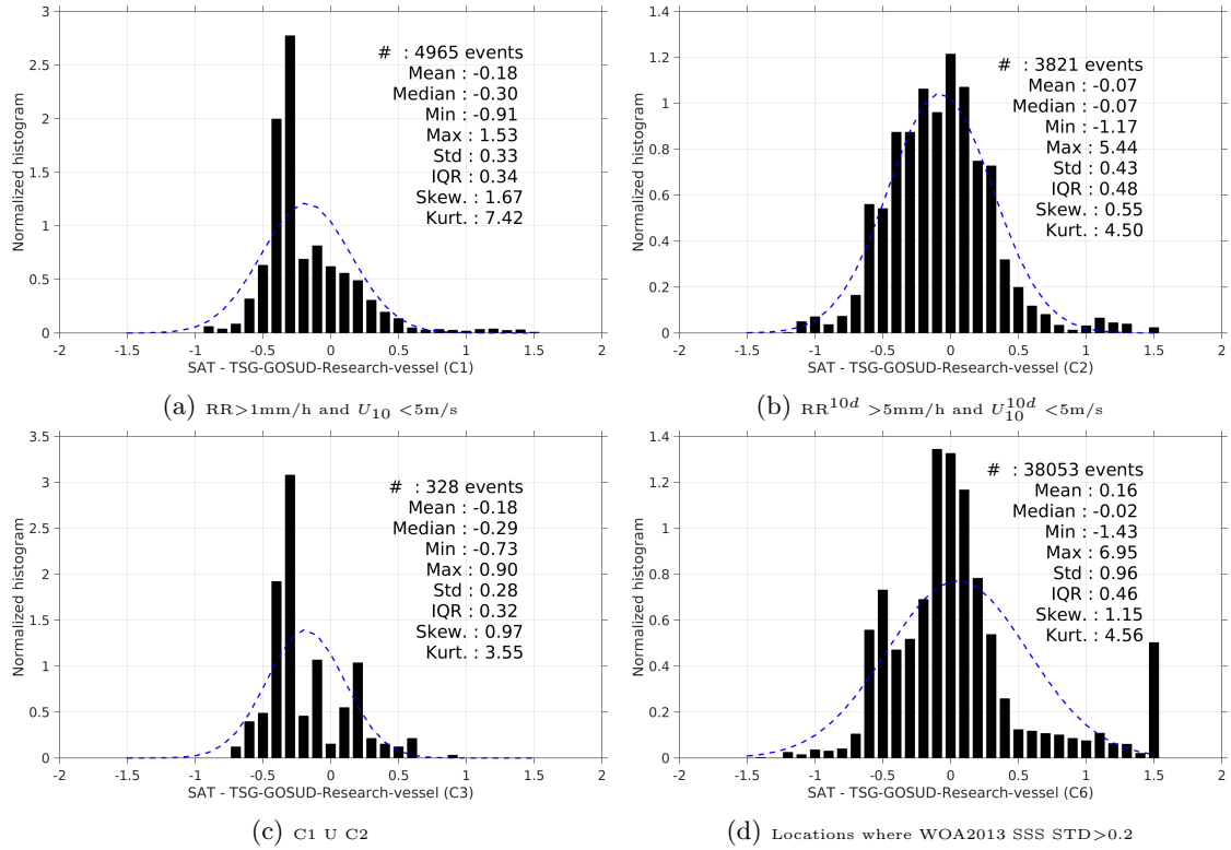
Figure 13: Normalized histogram of \Delta SSS (Aquarius-L4-IPRC-V4-WEEKLY - TSG-GOSUD-Research-vessel) for 6 different subdatasets corresponding to: RR > 1\text{mm/h} and U_{10} < 5\text{m/s} (a), RR^{10d} > 5\text{mm/h} and U_{10}^{10d} < 5\text{m/s} (b), C1 U C2 (c), Locations where WOA2013 SSS STD > 0.2 (d).
