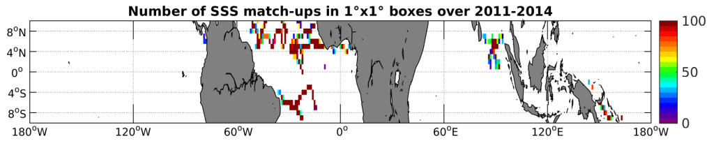
Figure 3: Number of SSS match-ups between Surface drifters SSS and the Aquarius-L4-IPRC-V4-WEEKLY SSS product for the Equatorial Ocean 10N-10S Pi-MEP region over 1^\circ \times 1^\circ boxes and for the full satellite product period.
