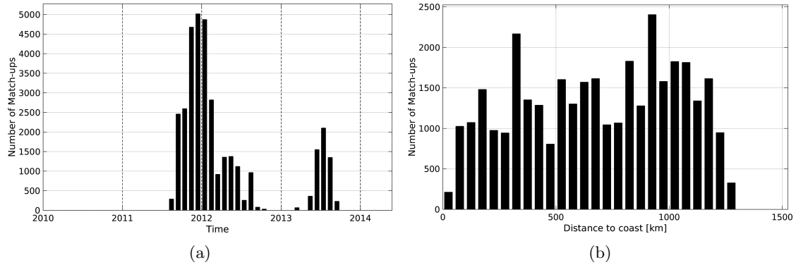
Figure 1: Number of match-ups between Surface drifters and Aquarius-L4-IPRC-V4-WEEKLY SSS as a function of time (a) and as function of the distance to coast (b) over the Equatorial Ocean 10N-10S Pi-MEP region and for the full satellite product period.
