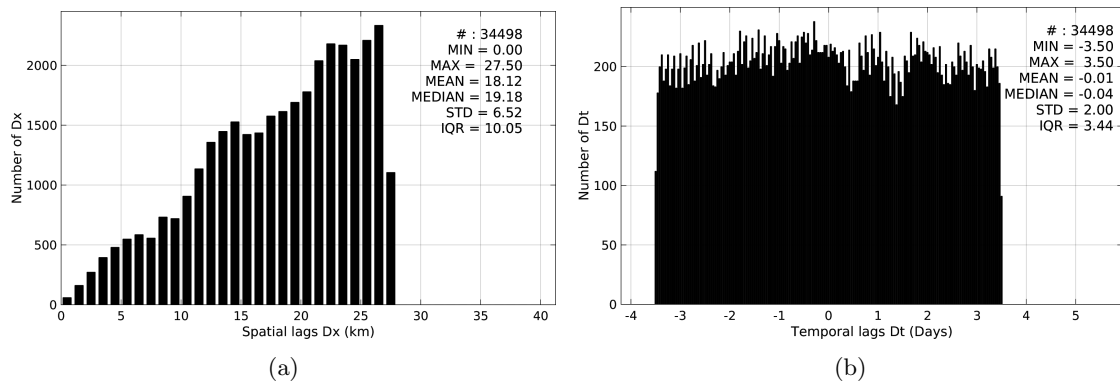
Figure 4: Histograms of the spatial (a) and temporal (b) lags between the time of the Surface drifters measurements and the date of the corresponding Aquarius-L4-IPRC-V4-WEEKLY SSS product.
