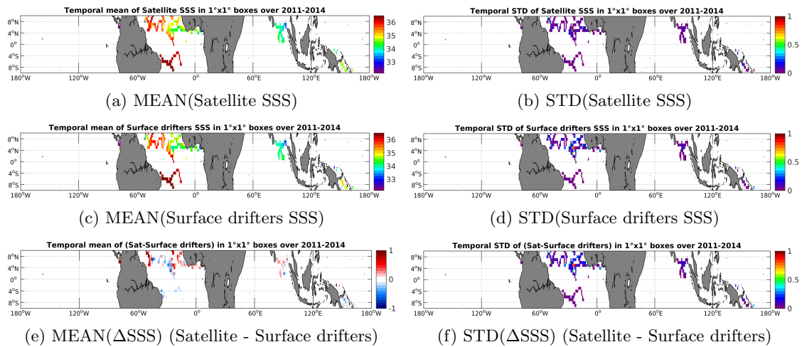
Figure 5: Temporal mean (left) and STD (right) of SSS from Aquarius-L4-IPRC-V4-WEEKLY (top), Surface drifters (middle), and of \Delta SSS (Satellite - Surface drifters). Only match-up pairs are used to generate these maps.
