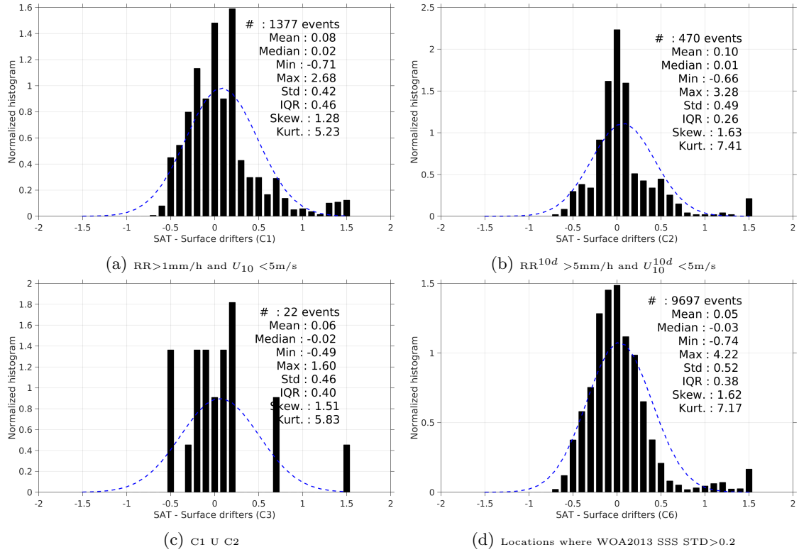
Figure 12: Normalized histogram of \Delta SSS (Aquarius-L4-IPRC-V4-WEEKLY - Surface drifters) for 6 different subdatasets corresponding to: RR > 1\text{mm/h} and U_{10} < 5\text{m/s} (a), RR^{10d} > 5\text{mm/h} and U_{10}^{10d} < 5\text{m/s} (b), C1 U C2 (c), Locations where WOA2013 SSS STD > 0.2 (d).
