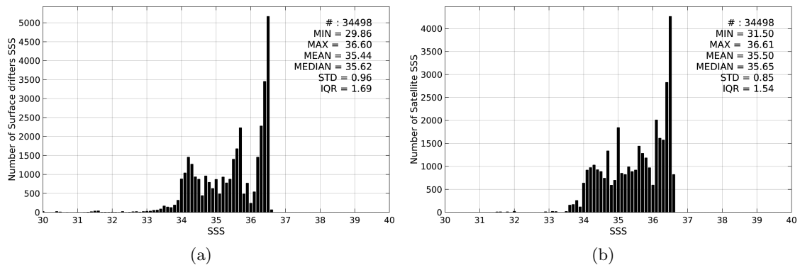
Figure 2: Histograms of SSS from Surface drifters (a) and Aquarius-L4-IPRC-V4-WEEKLY (b) considering all match-up pairs per bins of 0.1 over the Equatorial Ocean 10N-10S Pi-MEP region and for the full satellite product period.
