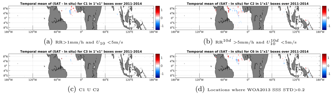
Figure 11: Temporal mean gridded over spatial boxes of size 1^\circ \times 1^\circ of \Delta SSS (Aquarius-L4-IPRC-V4-WEEKLY - Surface drifters) for 4 different subdatasets corresponding to: RR > 1\text{mm/h} and U_{10} < 5\text{m/s} (a), RR^{10d} > 5\text{mm/h} and U_{10}^{10d} < 5\text{m/s} (b), C1 U C2 (c), Locations where WOA2013 SSS STD > 0.2 (d).
