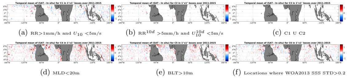
Figure 12: Temporal mean gridded over spatial boxes of size 1^\circ \times 1^\circ of \Delta SSS (Aquarius-L4-IPRC-V4-WEEKLY - Argo) for 6 different subdatasets corresponding to: RR > 1 mm/h and U_{10} < 5 m/s (a), RR^{10d} > 5 mm/h and U_{10}^{10d} < 5 m/s (b), C1 U C2 (c), MLD < 20 m (d), BLT > 10 m (e), Locations where WOA2013 SSS STD > 0.2 (f).
