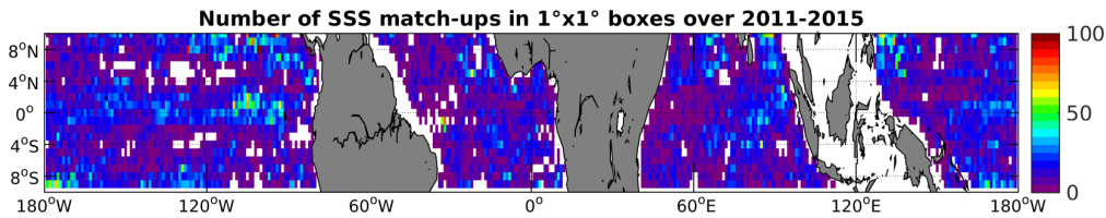
Figure 4: Number of SSS match-ups between Argo SSS and the Aquarius-L4-IPRC-V4-WEEKLY SSS product for the Equatorial Ocean 10N-10S Pi-MEP region over 1^\circ \times 1^\circ boxes and for the full satellite product period.
