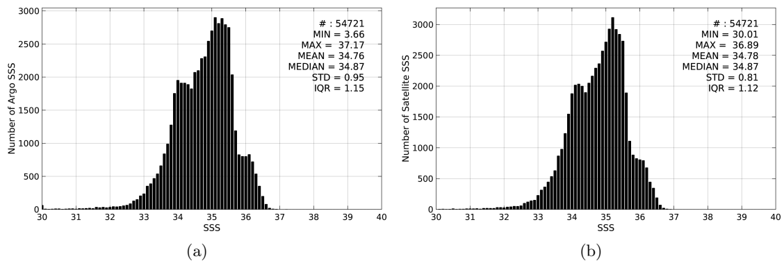
Figure 2: Histograms of SSS from Argo (a) and Aquarius-L4-IPRC-V4-WEEKLY (b) considering all match-up pairs per bins of 0.1 over the Equatorial Ocean 10N-10S Pi-MEP region and for the full satellite product period.
