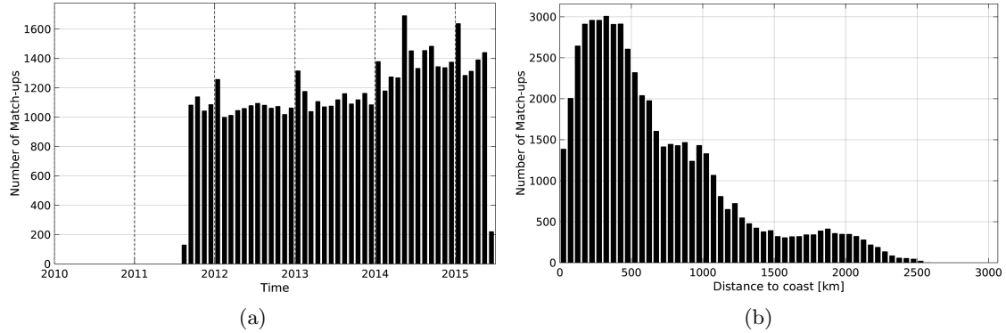
Figure 1: Number of match-ups between Argo and Aquarius-L4-IPRC-V4-WEEKLY SSS as a function of time (a) and as function of the distance to coast (b) over the Equatorial Ocean 10N-10S Pi-MEP region and for the full satellite product period.
