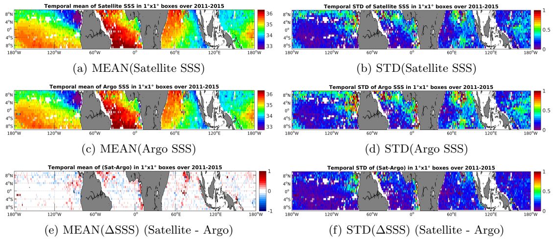
Figure 6: Temporal mean (left) and STD (right) of SSS from Aquarius-L4-IPRC-V4-WEEKLY (top), Argo (middle), and of \Delta SSS (Satellite - Argo). Only match-up pairs are used to generate these maps.
