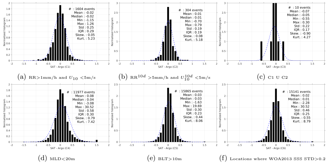
Figure 13: Normalized histogram of \Delta SSS (Aquarius-L4-IPRC-V4-WEEKLY - Argo) for 6 different subdatasets corresponding to: RR > 1 mm/h and U_{10} < 5 m/s (a), RR^{10d} > 5 mm/h and U_{10}^{10d} < 5 m/s (b), C1 U C2 (c), MLD < 20 m (d), BLT > 10 m (e), Locations where WOA2013 SSS STD > 0.2 (f).
