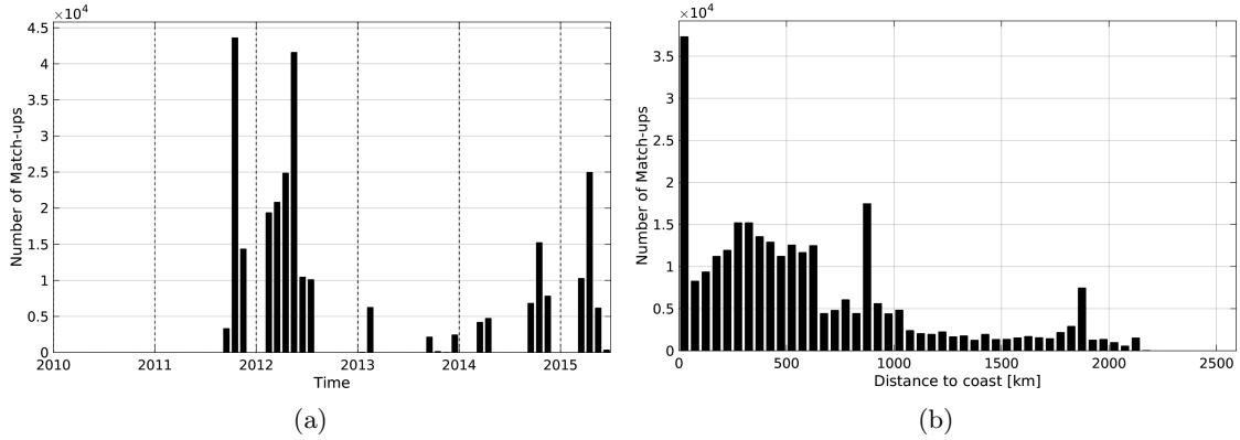
Figure 1: Number of match-ups between TSG-SAMOS and Aquarius-L4-IPRC-V4-MONTHLY SSS as a function of time (a) and as function of the distance to coast (b) over the Equatorial Ocean 10N-10S Pi-MEP region and for the full satellite product period.
