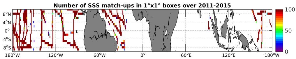
Figure 4: Number of SSS match-ups between TSG-SAMOS SSS and the Aquarius-L4-IPRC-V4-MONTHLY SSS product for the Equatorial Ocean 10N-10S Pi-MEP region over 1^\circ \times 1^\circ boxes and for the full satellite product period.
