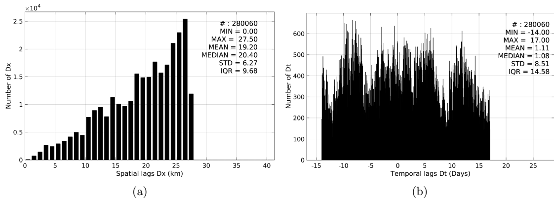
Figure 5: Histograms of the spatial (a) and temporal (b) lags between the time of the TSG-SAMOS measurements and the date of the corresponding Aquarius-L4-IPRC-V4-MONTHLY SSS product.
