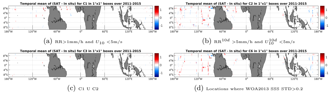
Figure 12: Temporal mean gridded over spatial boxes of size 1^\circ \times 1^\circ of \Delta SSS (Aquarius-L4-IPRC-V4-MONTHLY - TSG-SAMOS) for 4 different subdatasets corresponding to: RR > 1\text{mm/h} and U_{10} < 5\text{m/s} (a), RR^{10d} > 5\text{mm/h} and U_{10}^{10d} < 5\text{m/s} (b), C1 U C2 (c), Locations where WOA2013 SSS STD > 0.2 (d).
