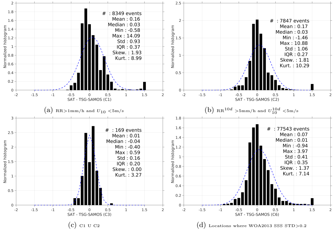
Figure 13: Normalized histogram of \Delta\text{SSS} (Aquarius-L4-IPRC-V4-MONTHLY - TSG-SAMOS) for 6 different subdatasets corresponding to: RR > 1mm/h and U_{10} < 5\text{m/s} (a), RR^{10d} > 5\text{mm/h} and U_{10}^{10d} < 5\text{m/s} (b), C1 U C2 (c), Locations where WOA2013 SSS STD > 0.2 (d).
