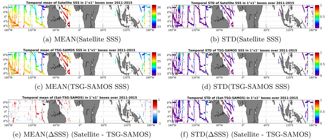
Figure 6: Temporal mean (left) and STD (right) of SSS from Aquarius-L4-IPRC-V4-MONTHLY (top), TSG-SAMOS (middle), and of \Delta SSS (Satellite - TSG-SAMOS). Only match-up pairs are used to generate these maps.
