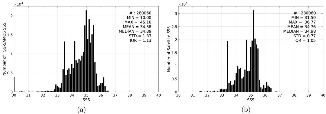
Figure 2: Histograms of SSS from TSG-SAMOS (a) and Aquarius-L4-IPRC-V4-MONTHLY (b) considering all match-up pairs per bins of 0.1 over the Equatorial Ocean 10N-10S Pi-MEP region and for the full satellite product period.
