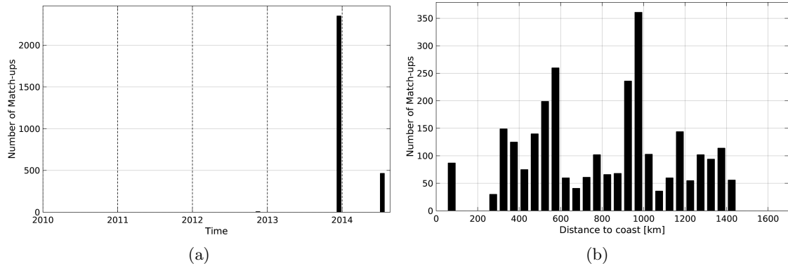
Figure 1: Number of match-ups between TSG-GOSUD-Sailing-ship and Aquarius-L4-IPRC-V4-MONTHLY SSS as a function of time (a) and as function of the distance to coast (b) over the Equatorial Ocean 10N-10S Pi-MEP region and for the full satellite product period.
