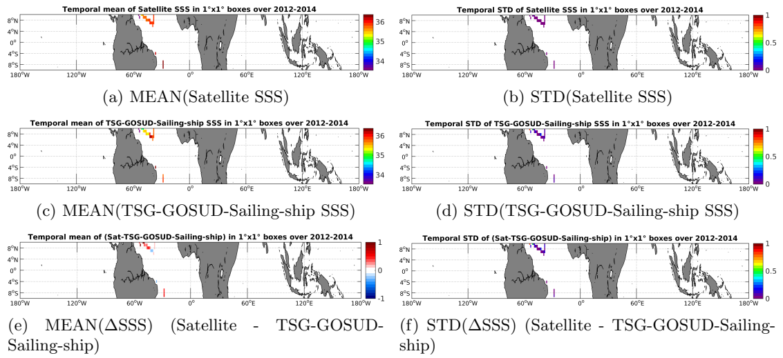
Figure 6: Temporal mean (left) and STD (right) of SSS from Aquarius-L4-IPRC-V4-MONTHLY (top), TSG-GOSUD-Sailing-ship (middle), and of \Delta SSS (Satellite - TSG-GOSUD-Sailing-ship). Only match-up pairs are used to generate these maps.
