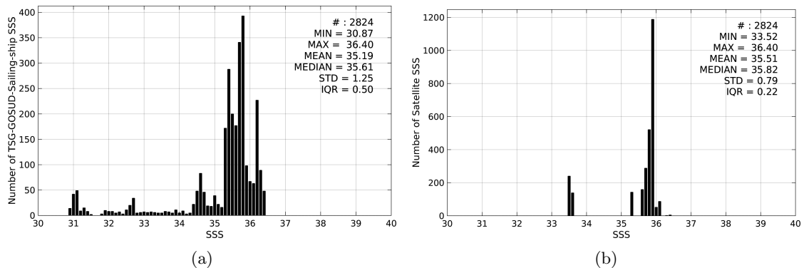
Figure 2: Histograms of SSS from TSG-GOSUD-Sailing-ship (a) and Aquarius-L4-IPRC-V4-MONTHLY (b) considering all match-up pairs per bins of 0.1 over the Equatorial Ocean 10N-10S Pi-MEP region and for the full satellite product period.
