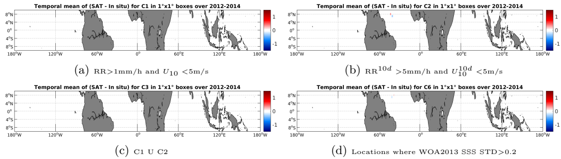
Figure 12: Temporal mean gridded over spatial boxes of size 1^\circ \times 1^\circ of \Delta SSS (Aquarius-L4-IPRC-V4-MONTHLY - TSG-GOSUD-Sailing-ship) for 4 different subdatasets corresponding to: RR > 1\text{mm/h} and U_{10} < 5\text{m/s} (a), RR^{10d} > 5\text{mm/h} and U_{10}^{10d} < 5\text{m/s} (b), C1 U C2 (c), Locations where WOA2013 SSS STD > 0.2 (d).
