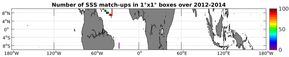
Figure 4: Number of SSS match-ups between TSG-GOSUD-Sailing-ship SSS and the Aquarius-L4-IPRC-V4-MONTHLY SSS product for the Equatorial Ocean 10N-10S Pi-MEP region over 1°x1° boxes and for the full satellite product period.
