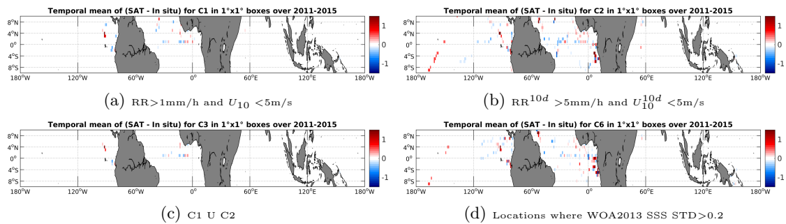
Figure 12: Temporal mean gridded over spatial boxes of size 1^\circ \times 1^\circ of \Delta SSS (Aquarius-L4-IPRC-V4-MONTHLY - TSG-GOSUD-Research-vessel) for 4 different subdatasets corresponding to:RR >1 mm/h and U_{10} < 5 m/s (a), RR ^{10d} > 5 mm/h and U_{10}^{10d} < 5 m/s (b), C1 U C2 (c),Locations where WOA2013 SSS STD >0.2 (d).
