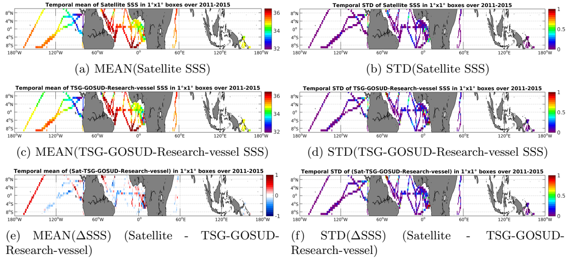
Figure 6: Temporal mean (left) and STD (right) of SSS from Aquarius-L4-IPRC-V4-MONTHLY (top), TSG-GOSUD-Research-vessel (middle), and of \Delta SSS (Satellite - TSG-GOSUD-Research-vessel). Only match-up pairs are used to generate these maps.
