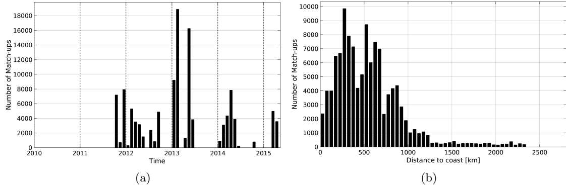
Figure 1: Number of match-ups between TSG-GOSUD-Research-vessel and Aquarius-L4-IPRC-V4-MONTHLY SSS as a function of time (a) and as function of the distance to coast (b) over the Equatorial Ocean 10N-10S Pi-MEP region and for the full satellite product period.
