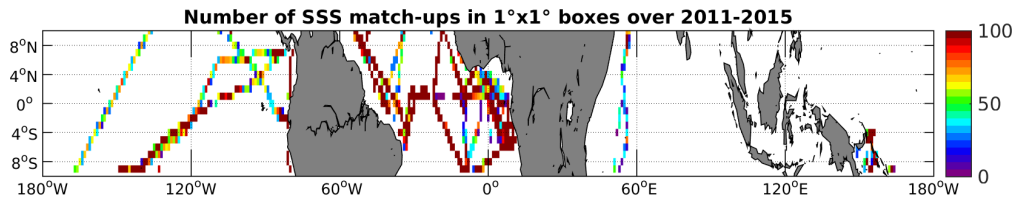
Figure 4: Number of SSS match-ups between TSG-GOSUD-Research-vessel SSS and the Aquarius-L4-IPRC-V4-MONTHLY SSS product for the Equatorial Ocean 10N-10S Pi-MEP region over 1^\circ \times 1^\circ boxes and for the full satellite product period.
