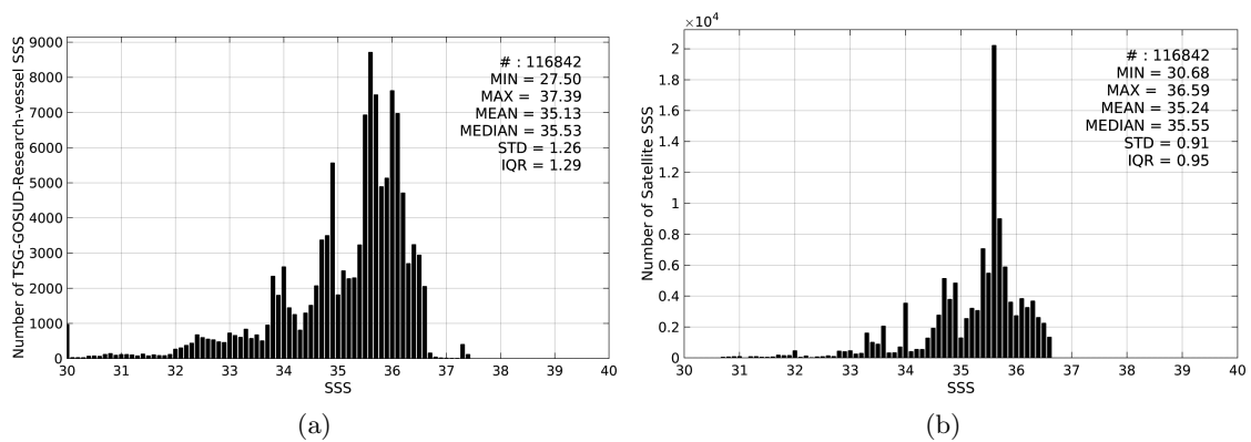
Figure 2: Histograms of SSS from TSG-GOSUD-Research-vessel (a) and Aquarius-L4-IPRC-V4-MONTHLY (b) considering all match-up pairs per bins of 0.1 over the Equatorial Ocean 10N-10S Pi-MEP region and for the full satellite product period.
