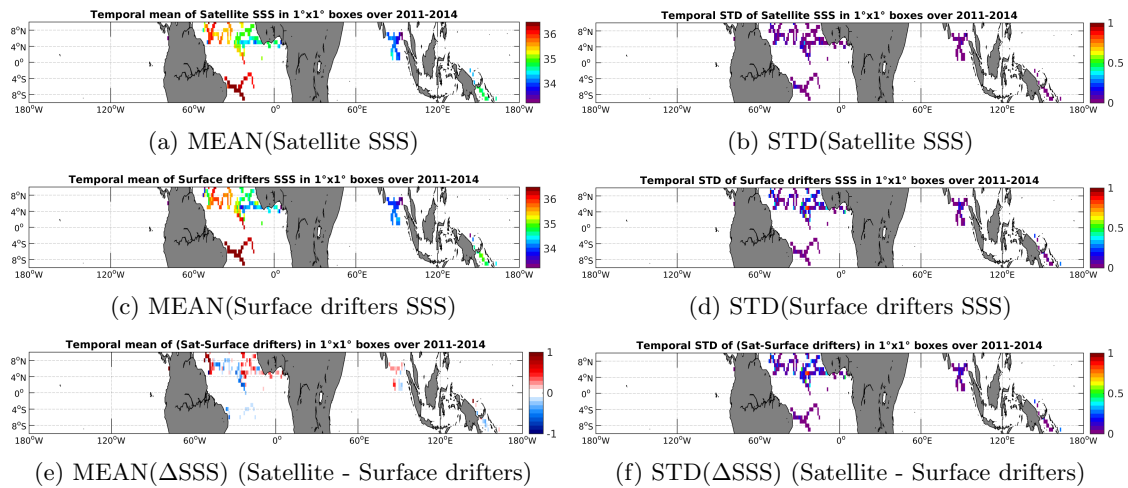
Figure 5: Temporal mean (left) and STD (right) of SSS from Aquarius-L4-IPRC-V4-MONTHLY (top), Surface drifters (middle), and of \Delta SSS (Satellite - Surface drifters). Only match-up pairs are used to generate these maps.
