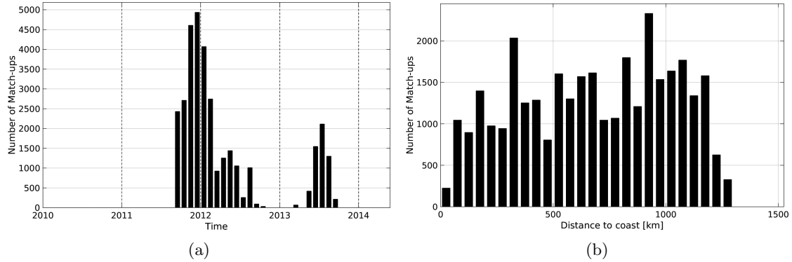
Figure 1: Number of match-ups between Surface drifters and Aquarius-L4-IIRC-V4-MONTHLY SSS as a function of time (a) and as function of the distance to coast (b) over the Equatorial Ocean 10N-10S Pi-MEP region and for the full satellite product period.
