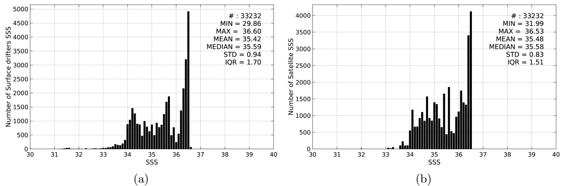
Figure 2: Histograms of SSS from Surface drifters (a) and Aquarius-L4-IIRC-V4-MONTHLY (b) considering all match-up pairs per bins of 0.1 over the Equatorial Ocean 10N-10S Pi-MEP region and for the full satellite product period.
