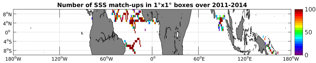
Figure 3: Number of SSS match-ups between Surface drifters SSS and the Aquarius-L4-IPRC-V4-MONTHLY SSS product for the Equatorial Ocean 10N-10S Pi-MEP region over 1^\circ \times 1^\circ boxes and for the full satellite product period.
