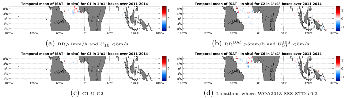
Figure 11: Temporal mean gridded over spatial boxes of size 1^\circ \times 1^\circ of \Delta SSS (Aquarius-L4-IPRC-V4-MONTHLY - Surface drifters) for 4 different subdatasets corresponding to: RR > 1\text{mm/h} and U_{10} < 5\text{m/s} (a), RR^{10d} > 5\text{mm/h} and U_{10}^{10d} < 5\text{m/s} (b), C1 U C2 (c), Locations where WOA2013 SSS STD > 0.2 (d).
