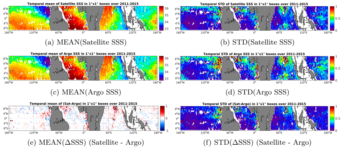
Figure 6: Temporal mean (left) and STD (right) of SSS from Aquarius-L4-IPRC-V4-MONTHLY (top), Argo (middle), and of \Delta SSS (Satellite - Argo). Only match-up pairs are used to generate these maps.
