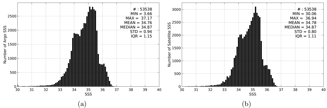
Figure 2: Histograms of SSS from Argo (a) and Aquarius-L4-IPRC-V4-MONTHLY (b) considering all match-up pairs per bins of 0.1 over the Equatorial Ocean 10N-10S Pi-MEP region and for the full satellite product period.
