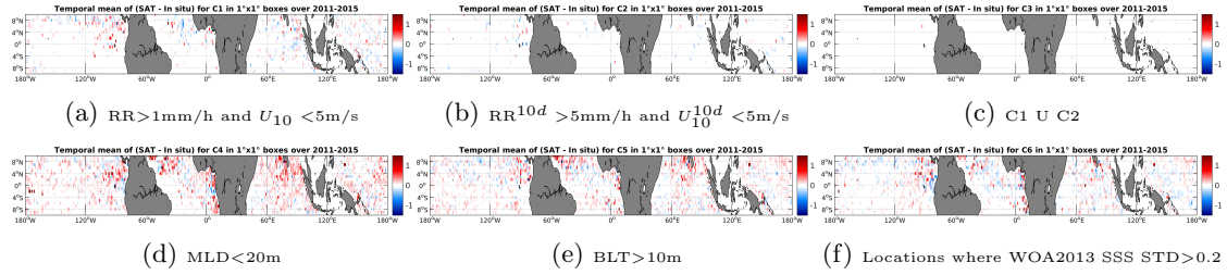
Figure 12: Temporal mean gridded over spatial boxes of size 1^\circ \times 1^\circ of \Delta SSS (Aquarius-L4-IPRC-V4-MONTHLY - Argo) for 6 different subdatasets corresponding to: RR > 1\text{mm/h} and U_{10} < 5\text{m/s} (a), RR^{10d} > 5\text{mm/h} and U_{10}^{10d} < 5\text{m/s} (b), C1 U C2 (c), MLD < 20\text{m} (d), BLT > 10\text{m} (e), Locations where WOA2013 SSS STD > 0.2 (f).
