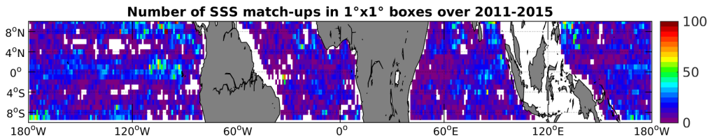
Figure 4: Number of SSS match-ups between Argo SSS and the Aquarius-L4-IPRC-V4-MONTHLY SSS product for the Equatorial Ocean 10N-10S Pi-MEP region over 1^\circ \times 1^\circ boxes and for the full satellite product period.
