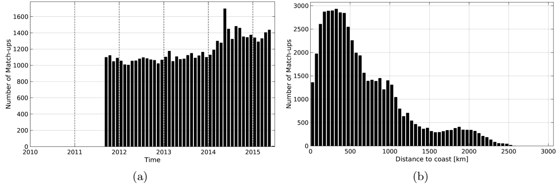
Figure 1: Number of match-ups between Argo and Aquarius-L4-IPRC-V4-MONTHLY SSS as a function of time (a) and as function of the distance to coast (b) over the Equatorial Ocean 10N-10S Pi-MEP region and for the full satellite product period.
