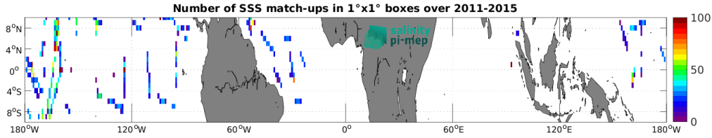
Figure 5: Number of SSS match-ups between TSG (SAMOS) SSS and the Aquarius SSS L3 OR v5 - 7-Day running (NASA-GSFC) SSS product for the Equatorial Ocean 10N-10S Pi-MEP region over 1^\circ \times 1^\circ boxes and for the full satellite product period.
