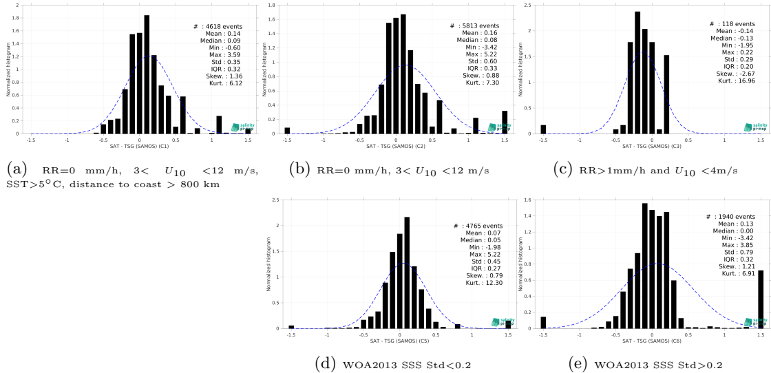
Figure 15: Normalized histogram of \Delta SSS (Aquarius SSS L3 OR v5 - 7-Day running (NASA-GSFC) - TSG (SAMOS)) for 5 different subdatasets corresponding to: RR=0 mm/h, 3 < U_{10} < 12 m/s, SST>5°C, distance to coast > 800 km (a), RR=0 mm/h, 3 < U_{10} < 12 m/s (b), RR>1mm/h and U_{10} < 4 m/s (c), WOA2013 SSS Std<0.2 (d), WOA2013 SSS Std>0.2 (e).
