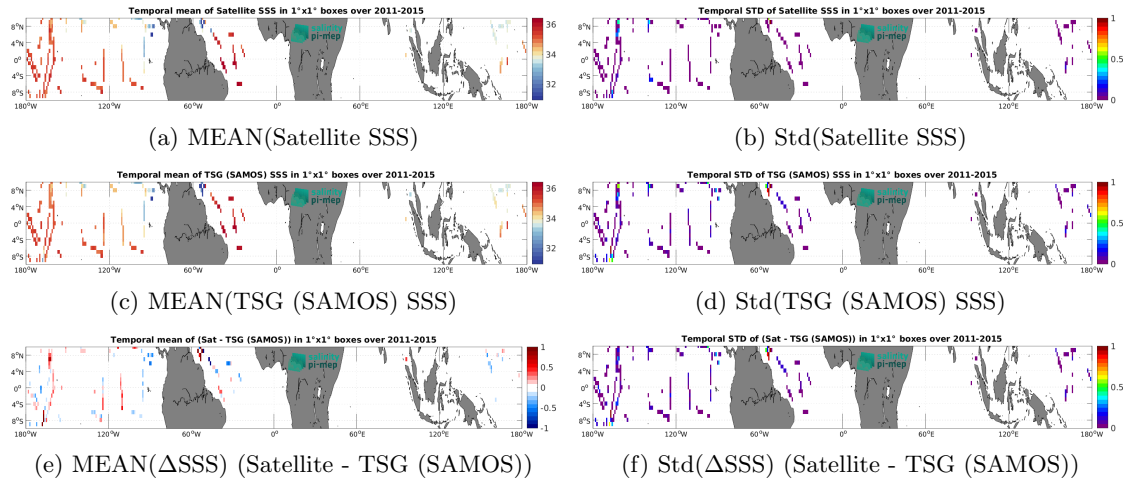
Figure 7: Temporal mean (left) and Std (right) of SSS from Aquarius SSS L3 OR v5 - 7-Day running (NASA-GSFC) (top), TSG (SAMOS) ( in situ ) (middle), and of \Delta SSS (Satellite - TSG (SAMOS)). Only match-up pairs are used to generate these maps.
