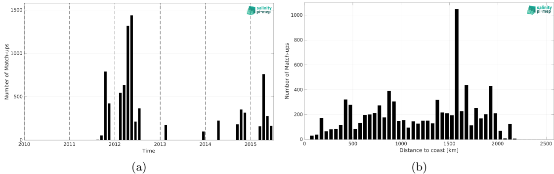
Figure 2: Number of match-ups between TSG (SAMOS) and Aquarius SSS L3 OR v5 - 7-Day running (NASA-GSFC) SSS as a function of time (a) and as function of the distance to coast (b) over the Equatorial Ocean 10N-10S Pi-MEP region and for the full satellite product period.
