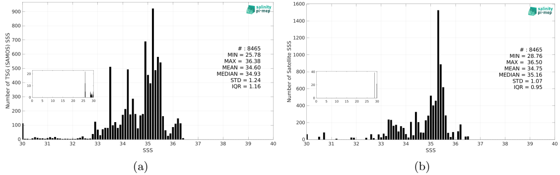
Figure 3: Histograms of SSS from TSG (SAMOS) (a) and Aquarius SSS L3 OR v5 - 7-Day running (NASA-GSFC) (b) considering all match-up pairs per bins of 0.1 over the Equatorial Ocean 10N-10S Pi-MEP region and for the full satellite product period.
