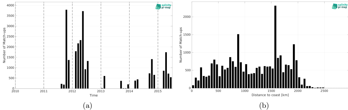
Figure 1: Number of match-ups between TSG (SAMOS) and Aquarius SSS L3 OR v5 - 7-Day running (NASA-GSFC) SSS as a function of time (a) and as function of the distance to coast (b) over the Equatorial Ocean 10N-10S Pi-MEP region and for the full satellite product period.
