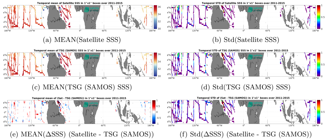
Figure 6: Temporal mean (left) and Std (right) of SSS from Aquarius SSS L3 OR v5 - 7-Day running (NASA-GSFC) (top), TSG (SAMOS) ( in situ ) (middle), and of \Delta SSS (Satellite - TSG (SAMOS)). Only match-up pairs are used to generate these maps.
