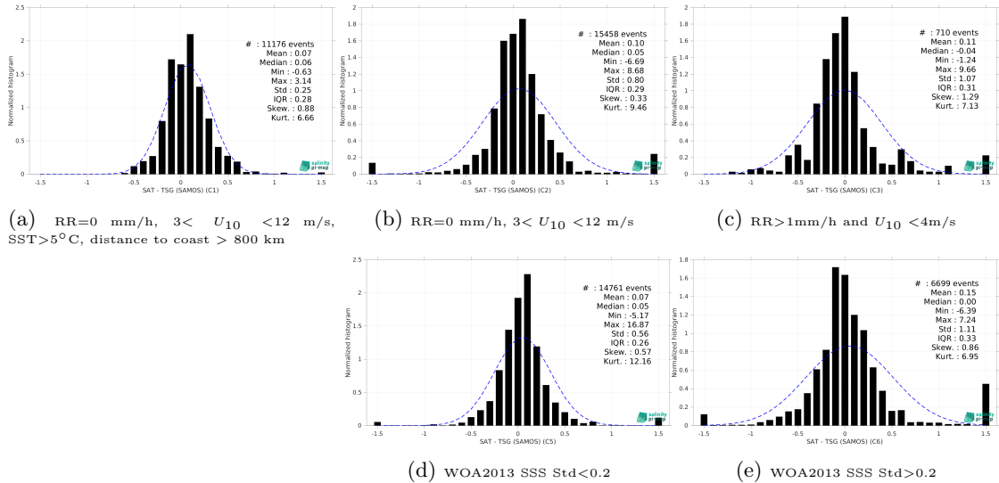
Figure 13: Normalized histogram of \Delta SSS (Aquarius SSS L3 OR v5 - 7-Day running (NASA-GSFC) - TSG (SAMOS)) for 5 different subdatasets corresponding to: RR=0 mm/h, 3 < U_{10} < 12 m/s, SST >5^\circ C, distance to coast > 800 km (a), RR=0 mm/h, 3 < U_{10} < 12 m/s (b), RR >1 mm/h and U_{10} < 4 m/s (c), WOA2013 SSS Std <0.2 (d), WOA2013 SSS Std >0.2 (e).
