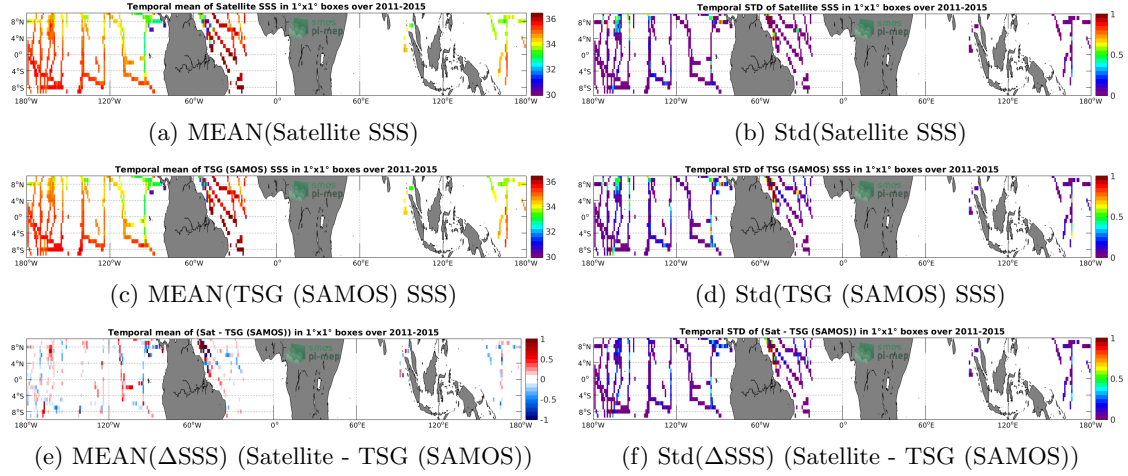
Figure 6: Temporal mean (left) and Std (right) of SSS from Aquarius SSS L3 OR v5 - 7-Day running (NASA-GSFC) (top), TSG (SAMOS) (middle), and of \Delta SSS (Satellite - TSG (SAMOS)). Only match-up pairs are used to generate these maps.
