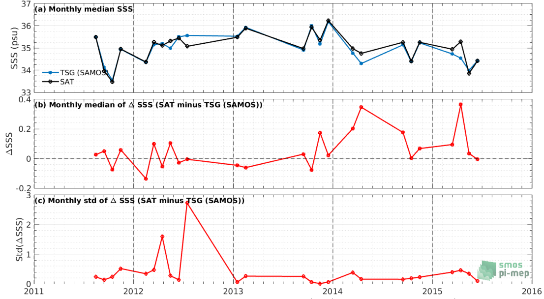
Figure 7: Time series of the monthly median SSS (top), median of \Delta\text{SSS} (Satellite - TSG (SAMOS)) and Std of \Delta\text{SSS} (Satellite - TSG (SAMOS)) over the Equatorial Ocean 10N-10S Pi-MEP region considering all match-ups collected by the Pi-MEP.
