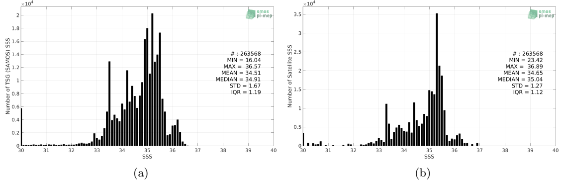
Figure 2: Histograms of SSS from TSG (SAMOS) (a) and Aquarius SSS L3 OR v5 - 7-Day running (NASA-GSFC) (b) considering all match-up pairs per bins of 0.1 over the Equatorial Ocean 10N-10S Pi-MEP region and for the full satellite product period.
