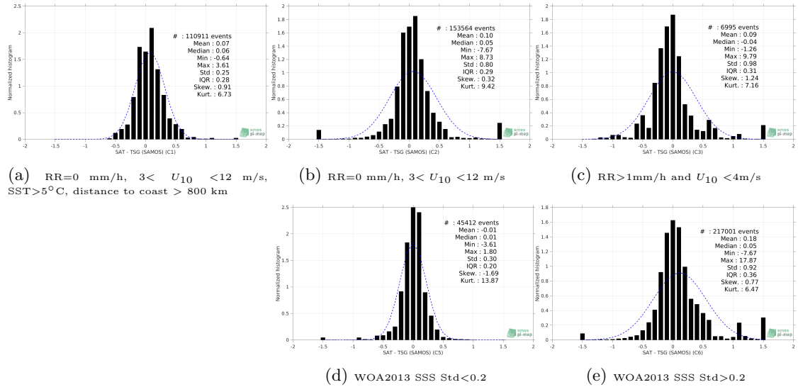
Figure 13: Normalized histogram of \Delta SSS (Aquarius SSS L3 OR v5 - 7-Day running (NASA-GSFC) - TSG (SAMOS)) for 5 different subdatasets corresponding to: RR=0 mm/h, 3 < U_{10} < 12 m/s, SST >5^\circ\text{C} , distance to coast > 800 km (a), RR=0 mm/h, 3 < U_{10} < 12 m/s (b), RR >1 mm/h and U_{10} < 4 m/s (c), WOA2013 SSS Std <0.2 (d), WOA2013 SSS Std >0.2 (e).
