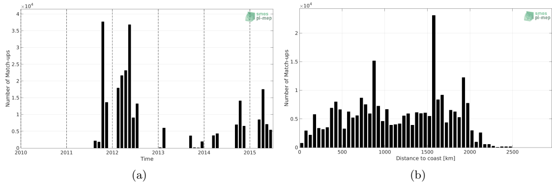
Figure 1: Number of match-ups between TSG (SAMOS) and Aquarius SSS L3 OR v5 - 7-Day running (NASA-GSFC) SSS as a function of time (a) and as function of the distance to coast (b) over the Equatorial Ocean 10N-10S Pi-MEP region and for the full satellite product period.
