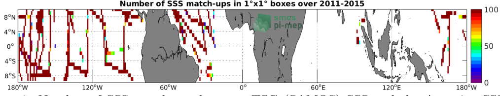
Figure 4: Number of SSS match-ups between TSG (SAMOS) SSS and the Aquarius SSS L3 OR v5 - 7-Day running (NASA-GSFC) SSS product for the Equatorial Ocean 10N-10S Pi-MEP region over 1^\circ \times 1^\circ boxes and for the full satellite product period.
