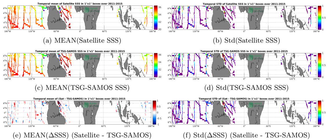
Figure 6: Temporal mean (left) and Std (right) of SSS from Aquarius-L3-OR-V5-7DAY-RUNNING-1DEG (top), TSG-SAMOS (middle), and of \Delta SSS (Satellite - TSG-SAMOS). Only match-up pairs are used to generate these maps.
