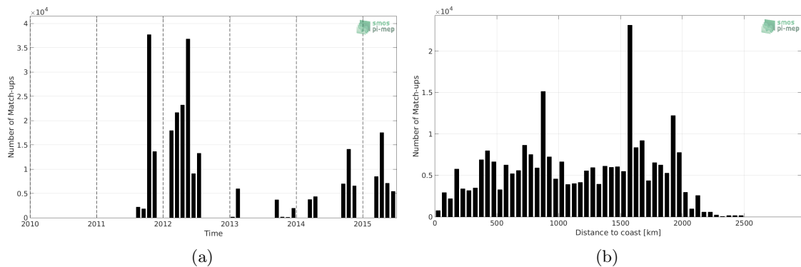
Figure 1: Number of match-ups between TSG-SAMOS and Aquarius-L3-OR-V5-7DAY-RUNNING-1DEG SSS as a function of time (a) and as function of the distance to coast (b) over the Equatorial Ocean 10N-10S Pi-MEP region and for the full satellite product period.
