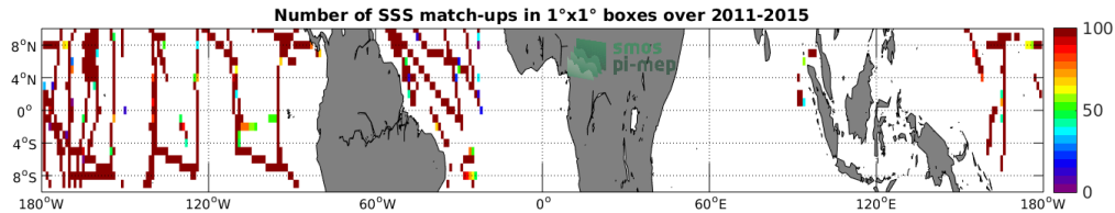
Figure 4: Number of SSS match-ups between TSG-SAMOS SSS and the Aquarius-L3-OR-V5-7DAY-RUNNING-1DEG SSS product for the Equatorial Ocean 10N-10S Pi-MEP region over 1°x1° boxes and for the full satellite product period.
