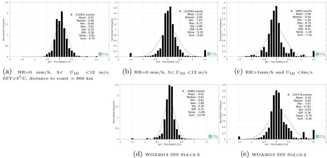
Figure 13: Normalized histogram of ΔSSS (Aquarius-L3-OR-V5-7DAY-RUNNING-1DEG - TSG-SAMOS) for 5 different subdatasets corresponding to: RR=0 mm/h, 3 < U_{10} < 12 m/s, SST>5°C, distance to coast > 800 km (a), RR=0 mm/h, 3 < U_{10} < 12 m/s (b), RR>1mm/h and U_{10} < 4 m/s (c), WOA2013 SSS Std<0.2 (d), WOA2013 SSS Std>0.2 (e).
