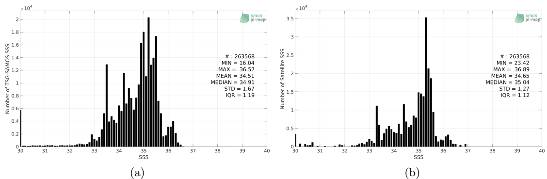
Figure 2: Histograms of SSS from TSG-SAMOS (a) and Aquarius-L3-OR-V5-7DAY-RUNNING-1DEG (b) considering all match-up pairs per bins of 0.1 over the Equatorial Ocean 10N-10S Pi-MEP region and for the full satellite product period.
