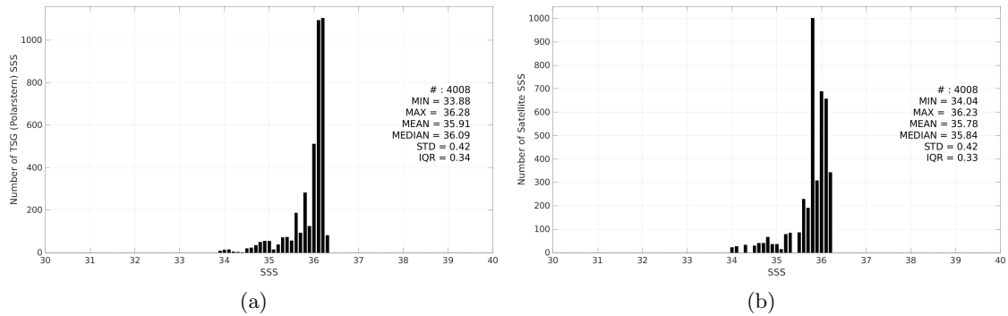
Figure 3: Histograms of SSS from TSG (Polarstern) (a) and Aquarius SSS L3 OR v5 - 7-Day running (NASA-GSFC) (b) considering all match-up pairs per bins of 0.1 over the Equatorial Ocean 10N-10S Pi-MEP region and for the full satellite product period.
