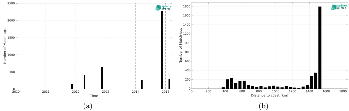
Figure 2: Number of match-ups between TSG (Polarstern) and Aquarius SSS L3 OR v5 - 7-Day running (NASA-GSFC) SSS as a function of time (a) and as function of the distance to coast (b) over the Equatorial Ocean 10N-10S Pi-MEP region and for the full satellite product period.
