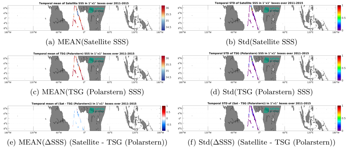
Figure 7: Temporal mean (left) and Std (right) of SSS from Aquarius SSS L3 OR v5 - 7-Day running (NASA-GSFC) (top), TSG (Polarstern) (middle), and of \Delta SSS (Satellite - TSG (Polarstern)). Only match-up pairs are used to generate these maps.
