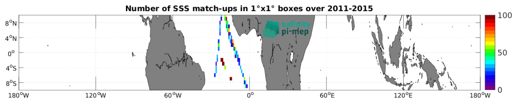
Figure 5: Number of SSS match-ups between TSG (Polarstern) SSS and the Aquarius SSS L3 OR v5 - 7-Day running (NASA-GSFC) SSS product for the Equatorial Ocean 10N-10S Pi-MEP region over 1^\circ \times 1^\circ boxes and for the full satellite product period.
