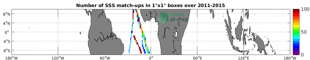
Figure 4: Number of SSS match-ups between TSG-POLARSTERN SSS and the Aquarius-L3-OR-V5-7DAY-RUNNING-1DEG SSS product for the Equatorial Ocean 10N-10S Pi-MEP region over 1^\circ \times 1^\circ boxes and for the full satellite product period.
