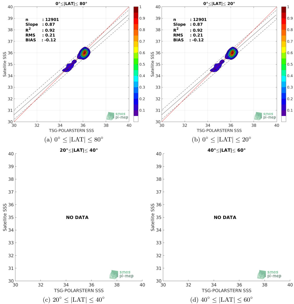
Figure 9: Contour maps of the concentration of Aquarius-L3-OR-V5-7DAY-RUNNING-1DEG SSS (y-axis) versus TSG-POLARSTERN SSS (x-axis) at match-up pairs for different latitude bands. For each plot, the red line shows x=y . The black thin and dashed lines indicate a linear fit through the data cloud and the \pm 95\% confidence levels, respectively. The number match-up pairs n , the slope and R^2 coefficient of the linear fit, the root mean square (RMS) and the mean bias between satellite and in situ data are indicated for each latitude band in each plots.
