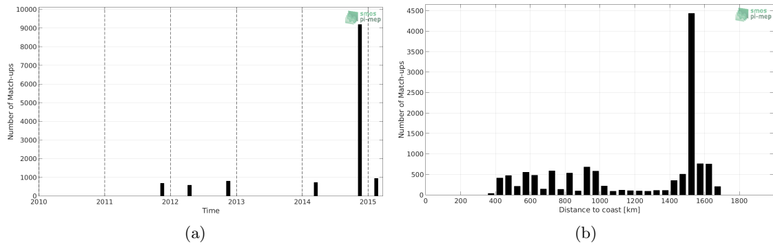
Figure 1: Number of match-ups between TSG-POLARSTERN and Aquarius-L3-OR-V5-7DAY-RUNNING-1DEG SSS as a function of time (a) and as function of the distance to coast (b) over the Equatorial Ocean 10N-10S Pi-MEP region and for the full satellite product period.
