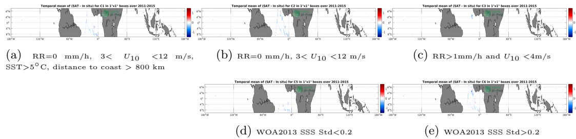
Figure 12: Temporal mean gridded over spatial boxes of size 1^\circ \times 1^\circ of \Delta SSS (Aquarius-L3-OR-V5-7DAY-RUNNING-1DEG - TSG-POLARSTERN) for 5 different subdatasets corresponding to:RR=0 mm/h, 3 < U_{10} < 12 m/s, SST >5^\circ C, distance to coast > 800 km (a), RR=0 mm/h, 3 < U_{10} < 12 m/s (b), RR >1 mm/h and U_{10} < 4 m/s (c), WOA2013 SSS Std <0.2 (d), WOA2013 SSS Std >0.2 (e).
