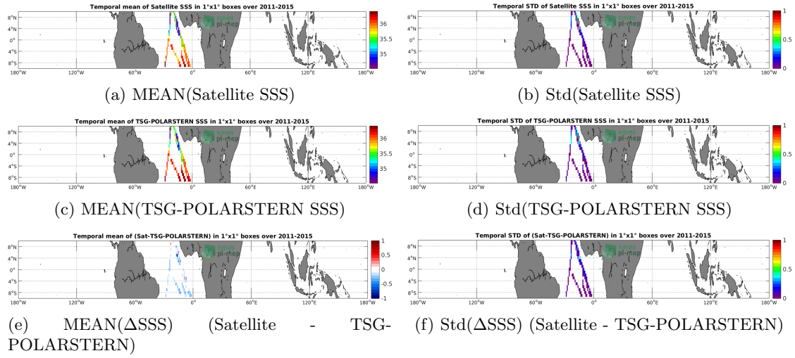
Figure 6: Temporal mean (left) and Std (right) of SSS from Aquarius-L3-OR-V5-7DAY-RUNNING-1DEG (top), TSG-POLARSTERN (middle), and of \Delta SSS (Satellite - TSG-POLARSTERN). Only match-up pairs are used to generate these maps.
