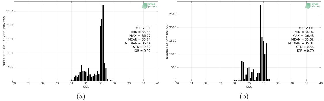
Figure 2: Histograms of SSS from TSG-POLARSTERN (a) and Aquarius-L3-OR-V5-7DAY-RUNNING-1DEG (b) considering all match-up pairs per bins of 0.1 over the Equatorial Ocean 10N-10S Pi-MEP region and for the full satellite product period.
