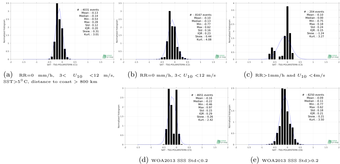
Figure 13: Normalized histogram of \Delta SSS (Aquarius-L3-OR-V5-7DAY-RUNNING-1DEG - TSG-POLARSTERN) for 5 different subdatasets corresponding to: RR=0 mm/h, 3 < U_{10} < 12 m/s, SST >5^\circ C, distance to coast > 800 km (a), RR=0 mm/h, 3 < U_{10} < 12 m/s (b), RR >1 mm/h and U_{10} < 4 m/s (c), WOA2013 SSS Std <0.2 (d), WOA2013 SSS Std >0.2 (e).
