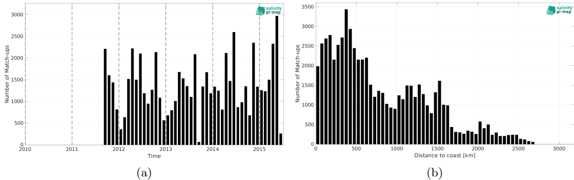
Figure 2: Number of match-ups between TSG (LEGOS-DM) and Aquarius SSS L3 OR v5 - 7-Day running (NASA-GSFC) SSS as a function of time (a) and as function of the distance to coast (b) over the Equatorial Ocean 10N-10S Pi-MEP region and for the full satellite product period.
