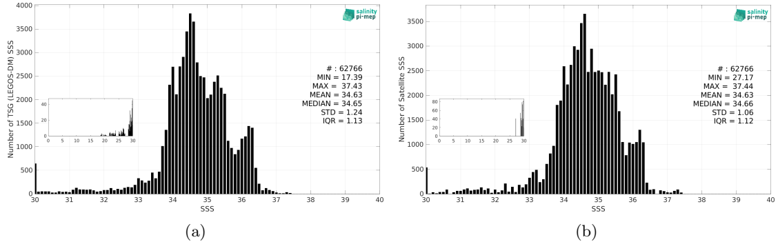
Figure 3: Histograms of SSS from TSG (LEGOS-DM) (a) and Aquarius SSS L3 OR v5 - 7-Day running (NASA-GSFC) (b) considering all match-up pairs per bins of 0.1 over the Equatorial Ocean 10N-10S Pi-MEP region and for the full satellite product period.
