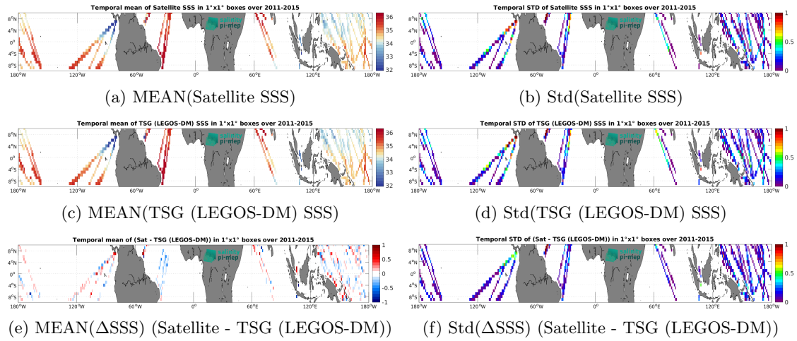
Figure 7: Temporal mean (left) and Std (right) of SSS from Aquarius SSS L3 OR v5 - 7-Day running (NASA-GSFC) (top), TSG (LEGOS-DM) (middle), and of \Delta SSS (Satellite - TSG (LEGOS-DM)). Only match-up pairs are used to generate these maps.
