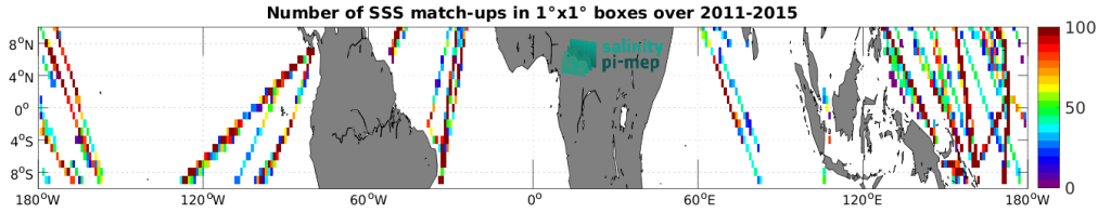
Figure 5: Number of SSS match-ups between TSG (LEGOS-DM) SSS and the Aquarius SSS L3 OR v5 - 7-Day running (NASA-GSFC) SSS product for the Equatorial Ocean 10N-10S Pi-MEP region over 1^\circ \times 1^\circ boxes and for the full satellite product period.
